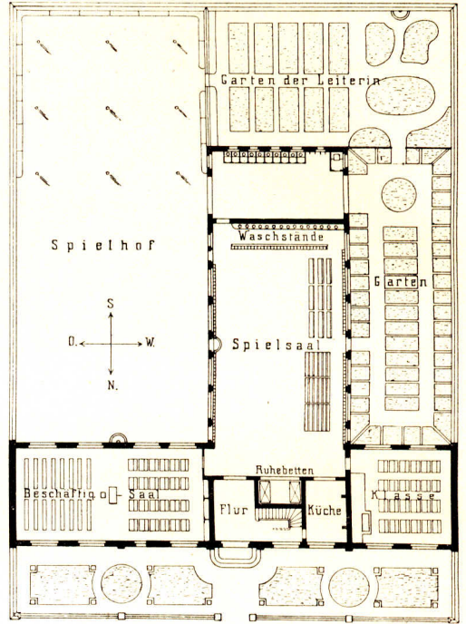
Erdgechofs.
