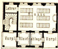
Erdgeschoss.
