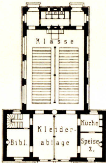
Erdgeschoss.
