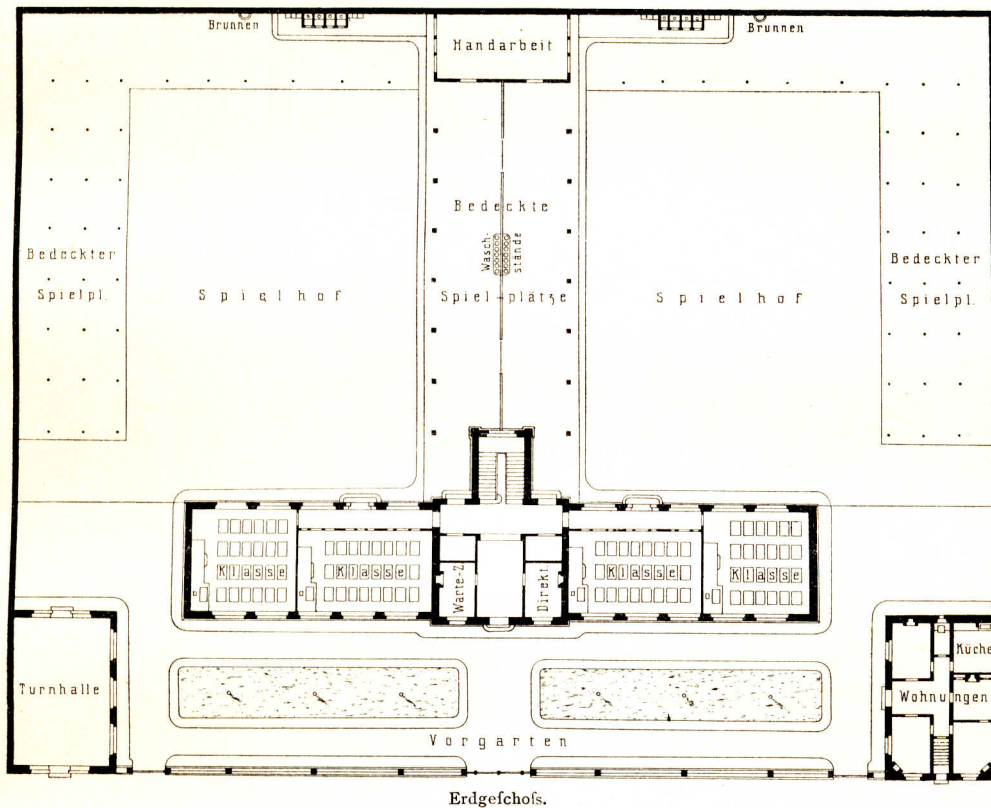
Erdgeschoss.
