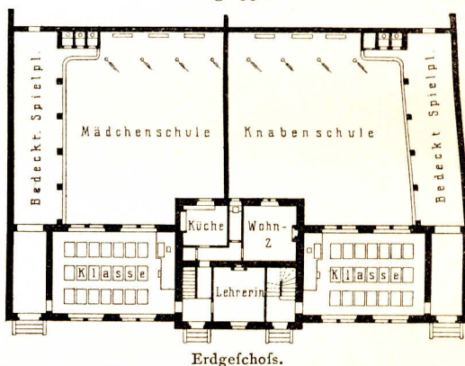
Erdgeschoss.
