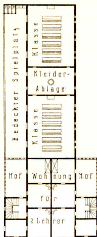
Erdgeschoss. \frac{1}{500} w. Gr.
