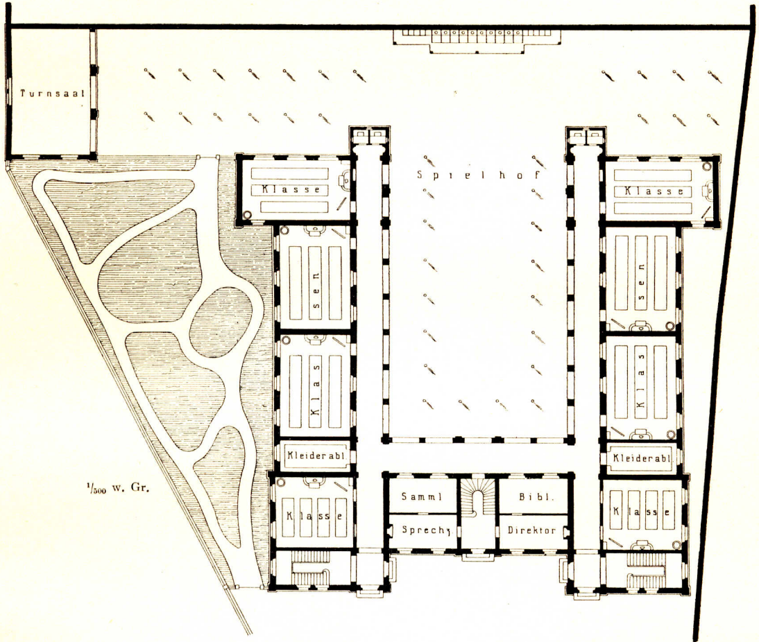
Erdgefchofs.
