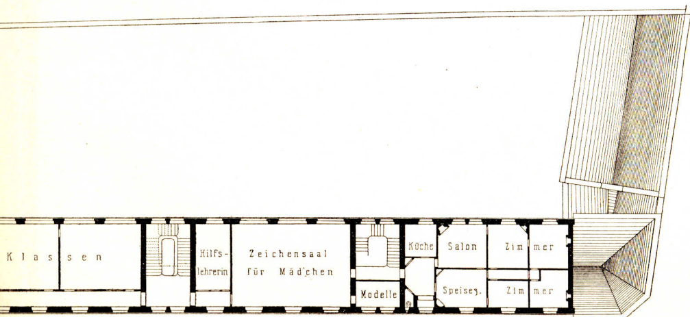
II. Ober- geschoss.
