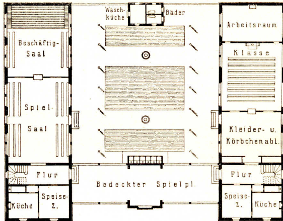
Erdgeschoss.
