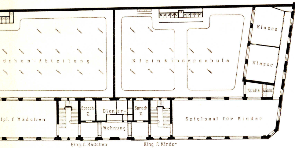
Erdgeschoss.
