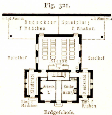
Erdgeschoss.
