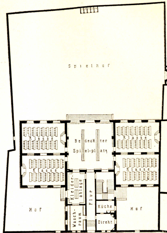
Erdgefchofs.
