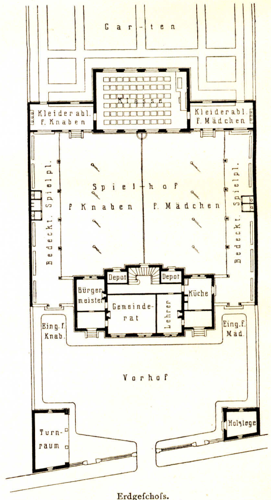
Erdgefchofs.
