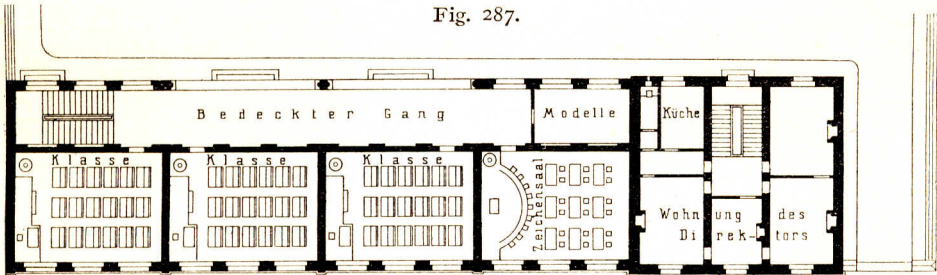
Erdgeschoss.
