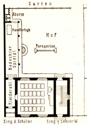
Erdgeschoss.
