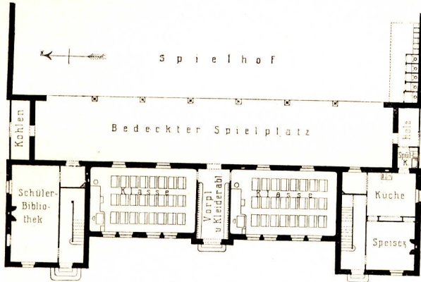
Erdgeschoss.
