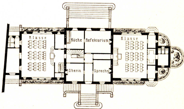
Erdgeschoss.
