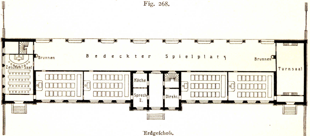
Erdgeschoss.
