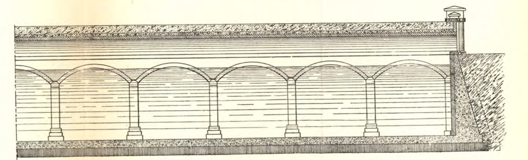
COVERED RESERVOIR: BRICK OR CONCRETE ARCHES ON COLUMNS.
