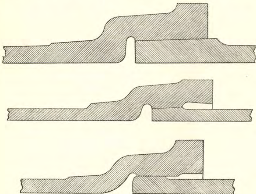
Figs. 200, 201, 202.—Spiggot and socket pipes with turned and bored joints.
