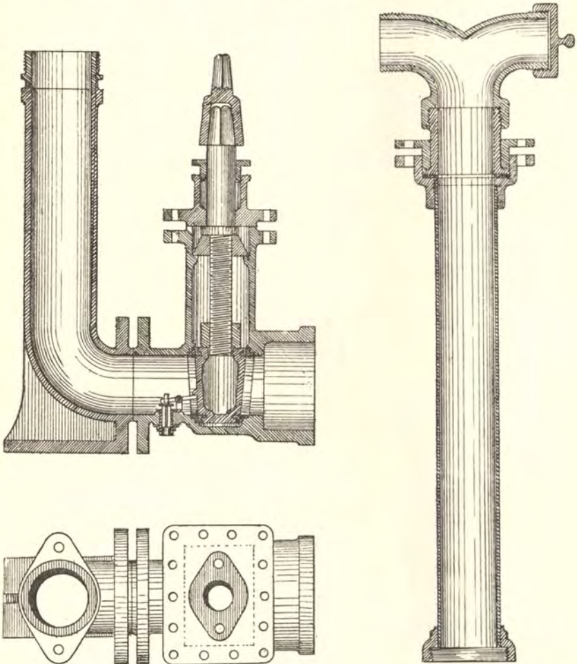
Fig. 193.—Stand-pipe for sluice-valve hydrant.
