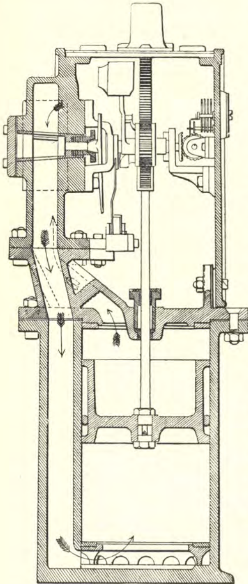
Fig. 232.—Kennedy's patent water meter.
