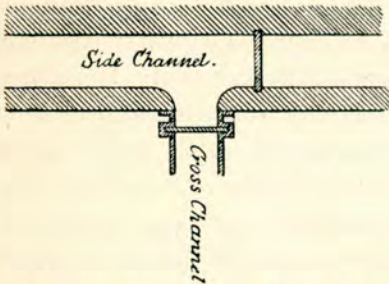
Fig. 58.—Side and cross channels of settling tanks.
