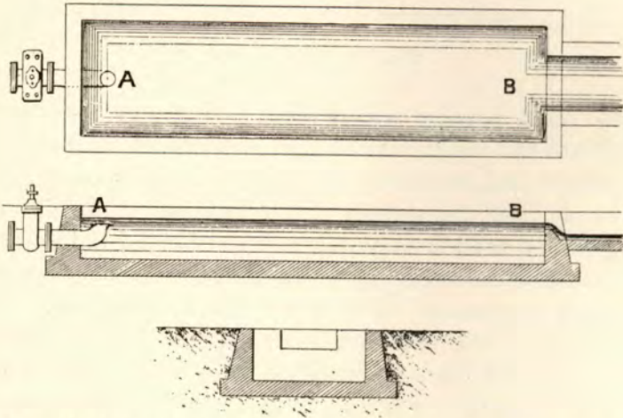
Figs. 125, 126 and 127.—"Canal" sand-washer (in plan and sections).
