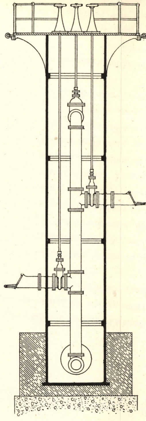
Figs. 39, 40.—Vertical Sections.
