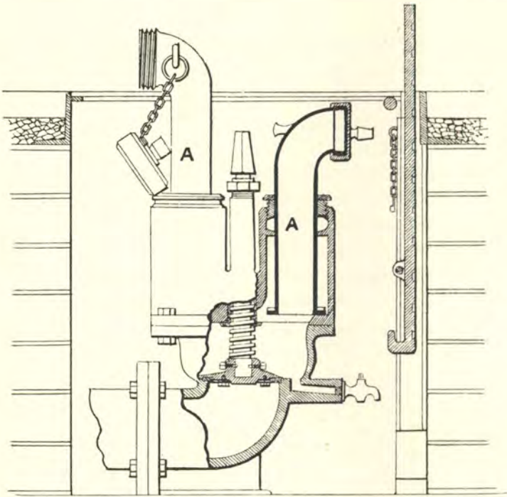
Fig. 189.—Merryweather's hydrant.
