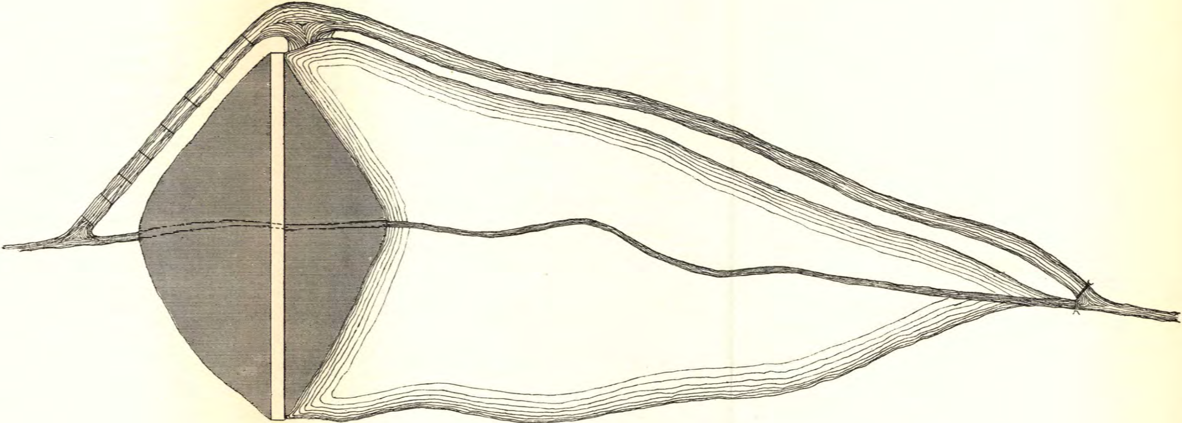
FIG. 46.—IMPOUNDING RESERVOIR, IN PLAN, WITH WASTE WEIR AND FLOOD CHANNEL.
