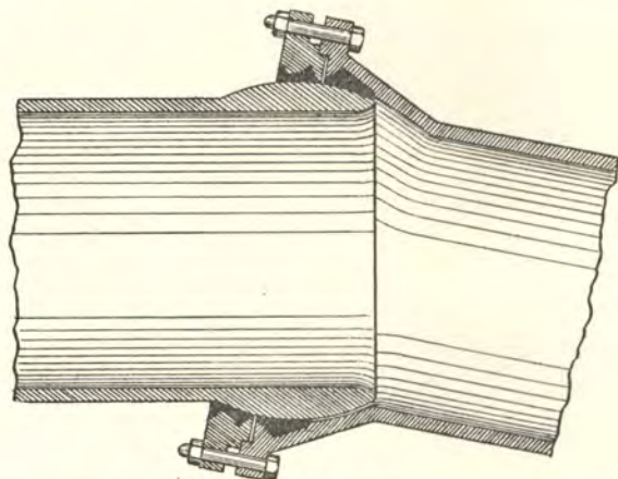
Fig. 209.—Waterpipe with ball and socket joint (Fanning).
