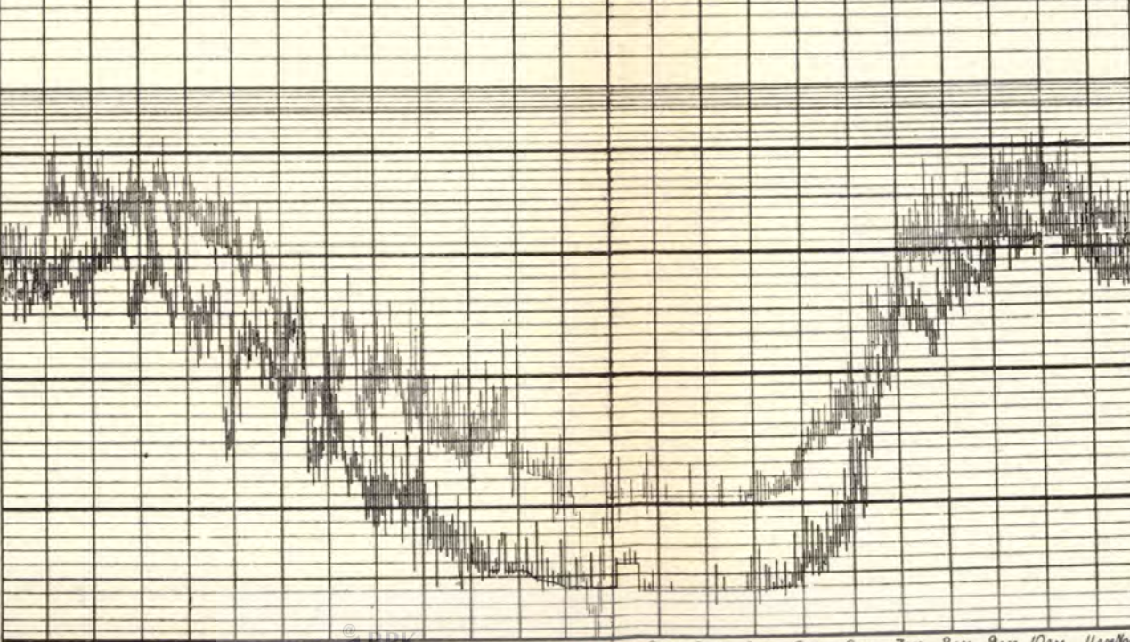
Fig. 229 CHORLEY Example of Waste Water Meter Diagrams from a District of 4,095 Persons. Fine Diagram Dec. 1881 night inspection under WWM system. Thick Diagram Jan. 1882 after repair of leaks detected by one night inspection. SAVING 3.70 3.95
