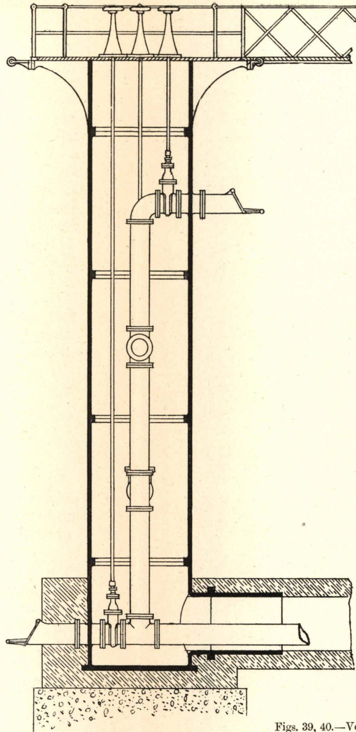
Figs. 39, 40.—Vertical Sections.
