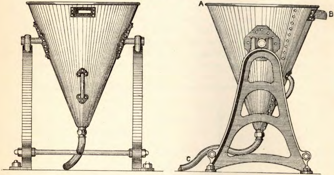
Figs. 123 and 124.—Walker's patent sand-washing apparatus.
