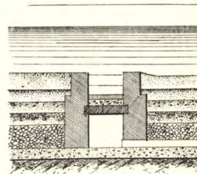
Fig. 105.—Section across the Gathering Drain.
