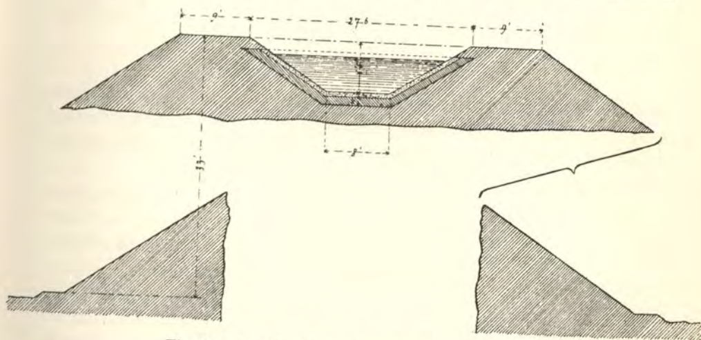
Fig. 150.—Section of open channel embanked—scale \frac{1}{200} .
