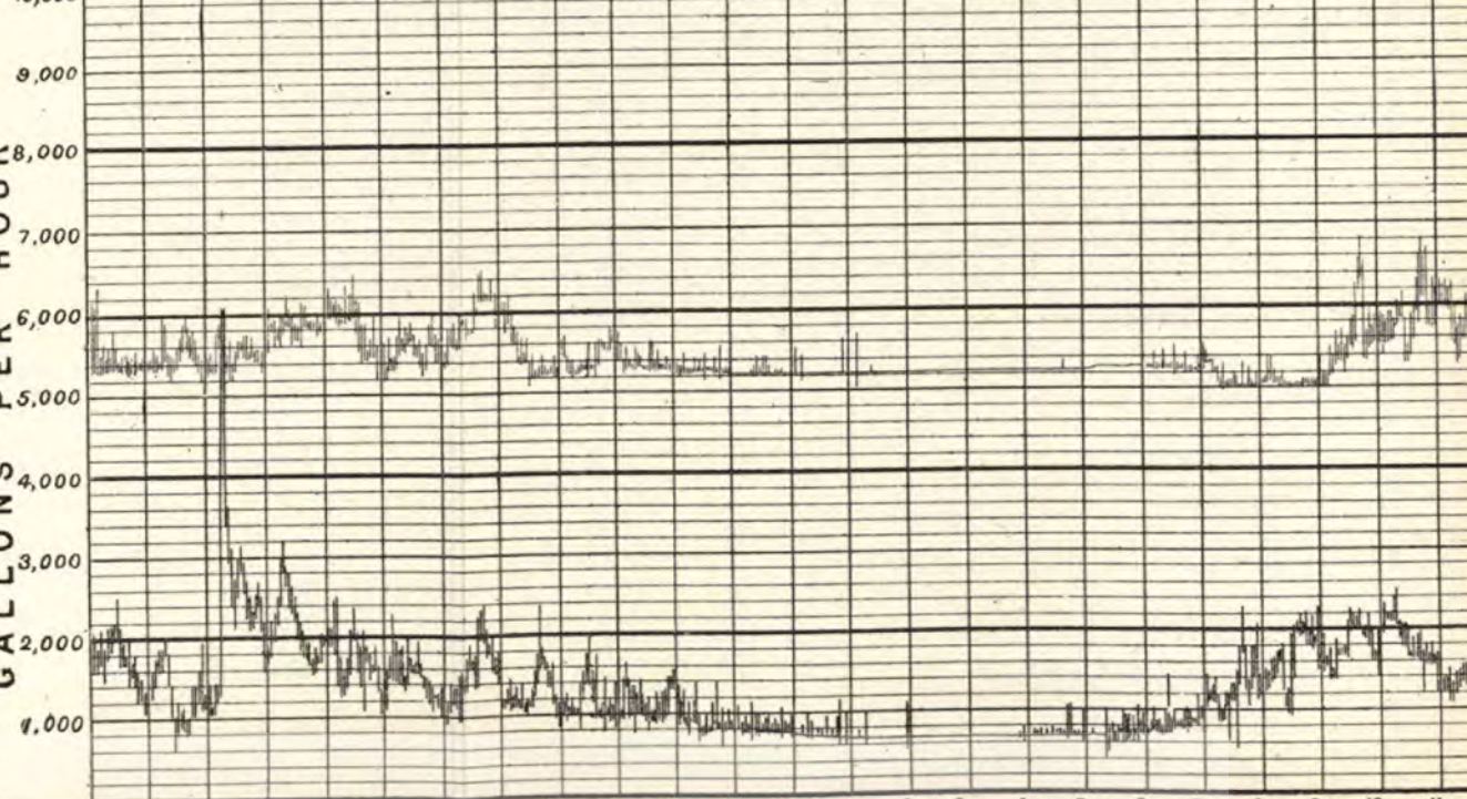
Fig. 230 LONDON (LAMBETH WATER CO.) Example of Waste Water Meter Diagrams from a District of 2,744 Persons. Fine Diagram Sep. 1881 before application of WWM system. Thick Diagram Nov. 1881 after application of WWM system. SAVING 47.0 10.9 36.1
