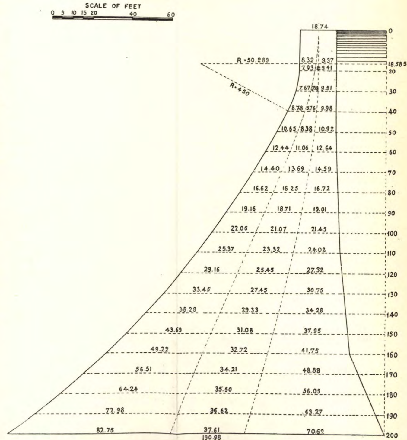
Fig. 53.—Practical Profile No. 3.
