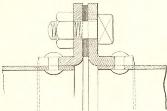
Fig. 218.—Stamped steel flanged joint.
