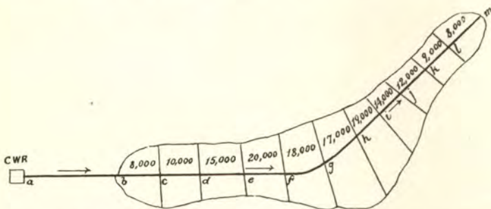
Fig. 179.—Diagram illustrating arrangement of distributing mains.
