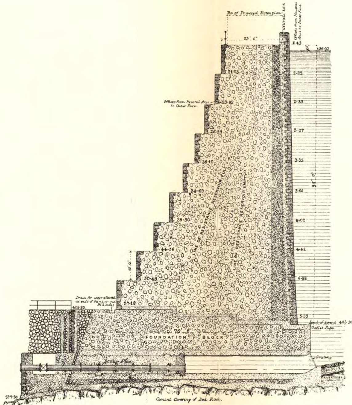
FIG. 54.—TYTAM DAM, HONGKONG: SECTION THROUGH SCOUR PIPE.
