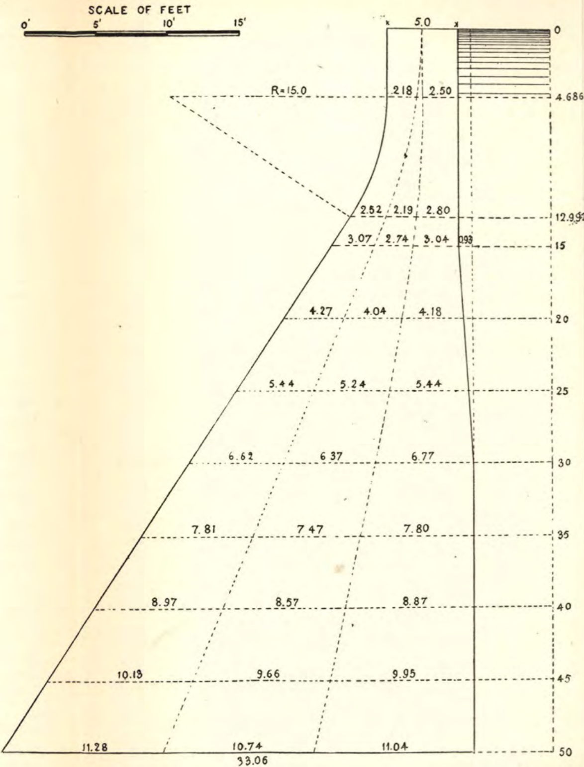
Fig. 51.—Practical Profile No. 1.
