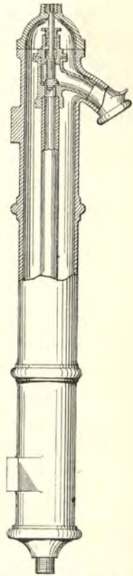
Fig. 244. — Blakeborough's stand pillar.
