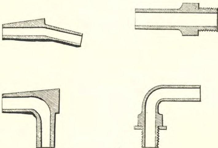
Figs. 245, 246.—Tapered ferrules for connecting waterpipes.
