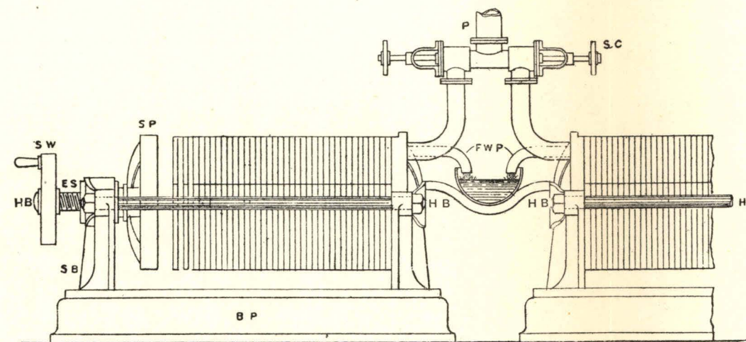
Fig. 136.—Filter-press.
