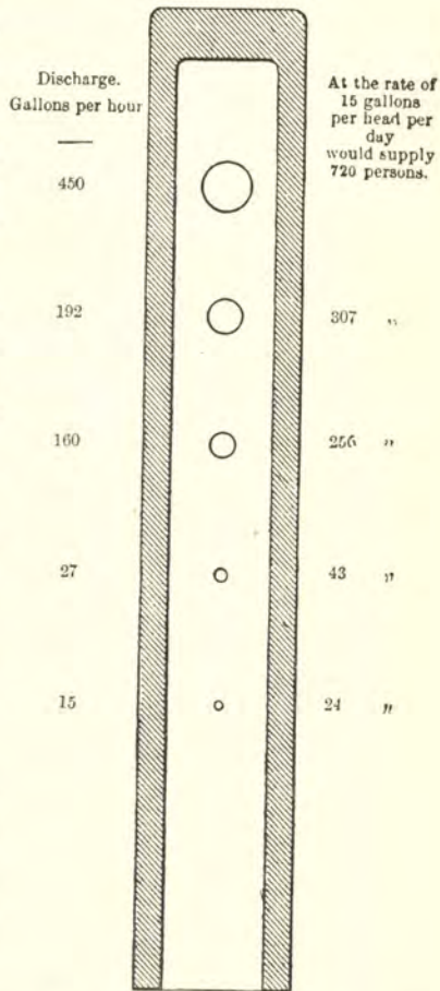
Fig. 221.—Results of experiments on the flow of water through circular holes in ½ in. lead-pipe under pressure of 45 lbs. per sq. in., showing number of persons who might be supplied by the discharge through flaws of various sizes.
