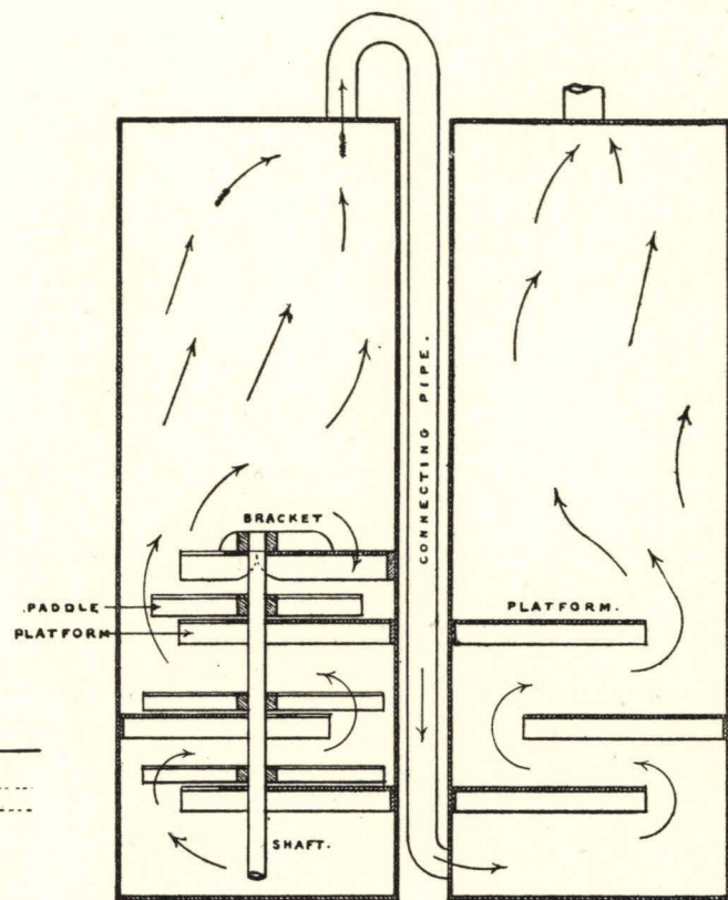
Fig. 133.—Longitudinal Section of Precipitating Tanks.
