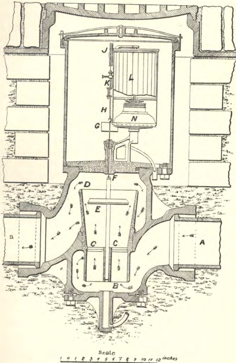
Fig. 223.—Mr. G. F. Deacon's "District" water meter.
