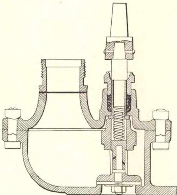
Fig. 195.—Screw-down hydrant (second example).
