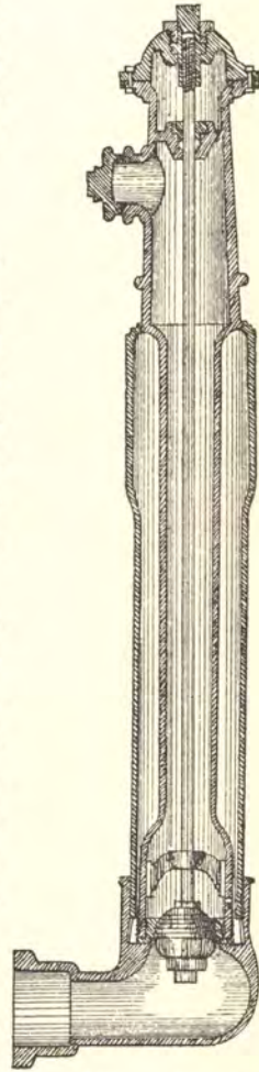
Fig. 188. — American form of pillar hydrant (Fanning).
