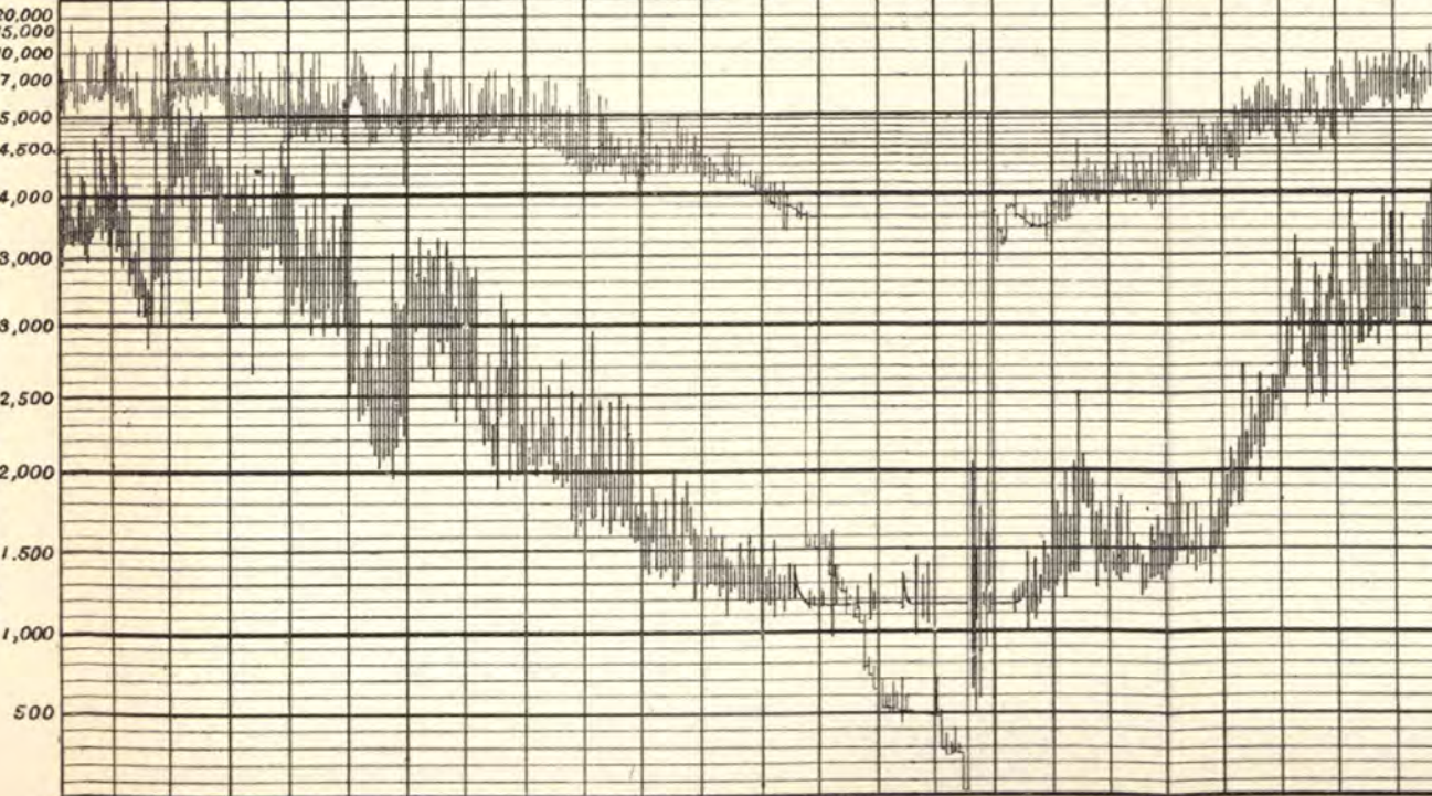
Fig. 228 LIVERPOOL Example of Waste Water Meter Diagrams from a District of 5,500 Persons. Fine Diagram Jan. 1882 night inspection under WWM system. Thick Diagram 2 following days after repair of leak repaired at 12.50 p.m. & before repair of other defects. SAVING 10.32 11.56
