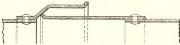
Fig. 220.—The Riley patent joint for water-pipes.
