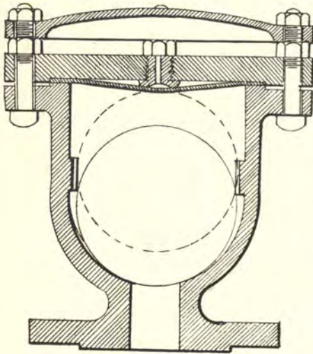
Fig. 239.—Air valve for waterpipe.
