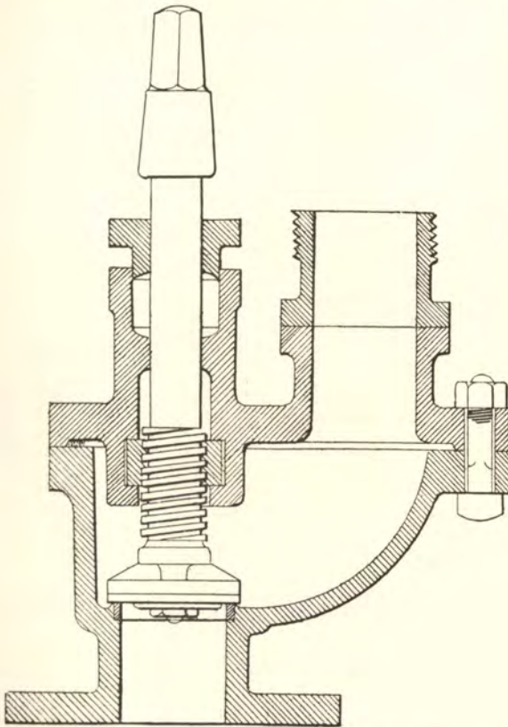
Fig. 194.—Screw-down hydrant (first example).
