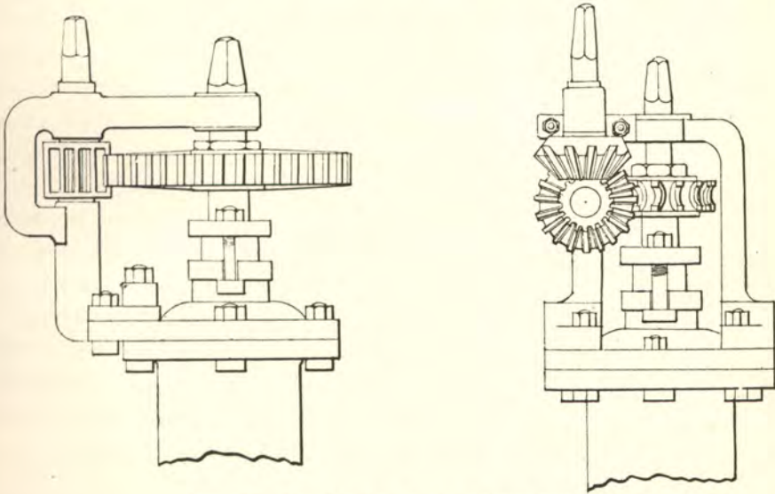
Figs. 237, 238.—Gear for opening sluice valves.
