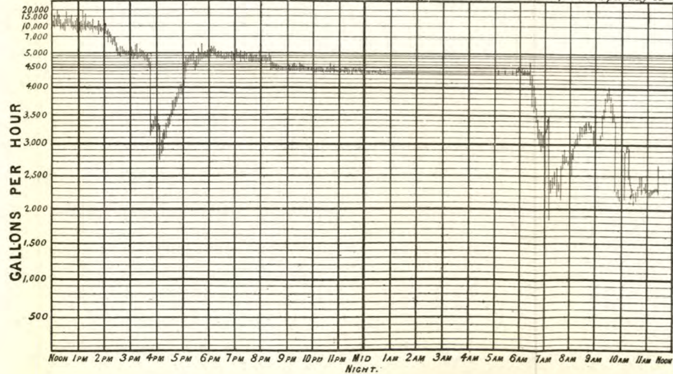
Fig. 226 LONDON LAMBETH WATER CO Example of a Waste Water Meter Diagram April 1882 from a District of 1,256 Persons, showing a partial night inspection, commenced at 6.25 a.m. being the first after the fixing of the Meter
