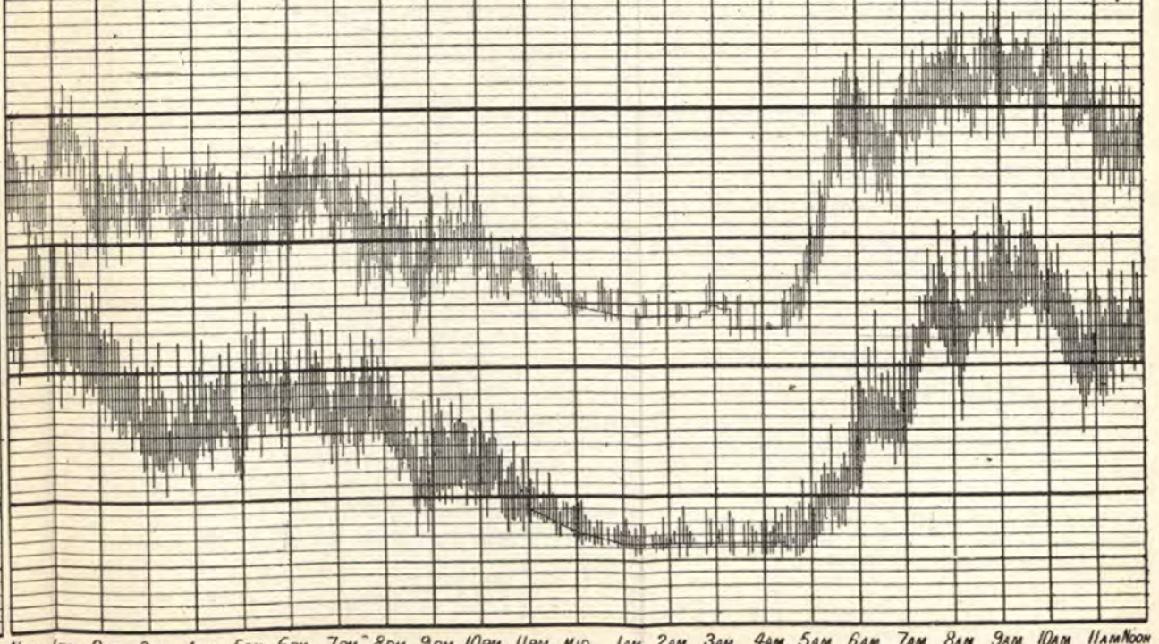
Fig. 231 BOSTON U.S.A. Example of Waste Water Meter Diagrams from a District of 2,810 Persons. Fine Diagram May 1881 before application of WWM system. Thick Diagram Dec. 1881 after application of WWM system. SAVING 53.5 39.7 26.4 10.6 27.1 28.5
