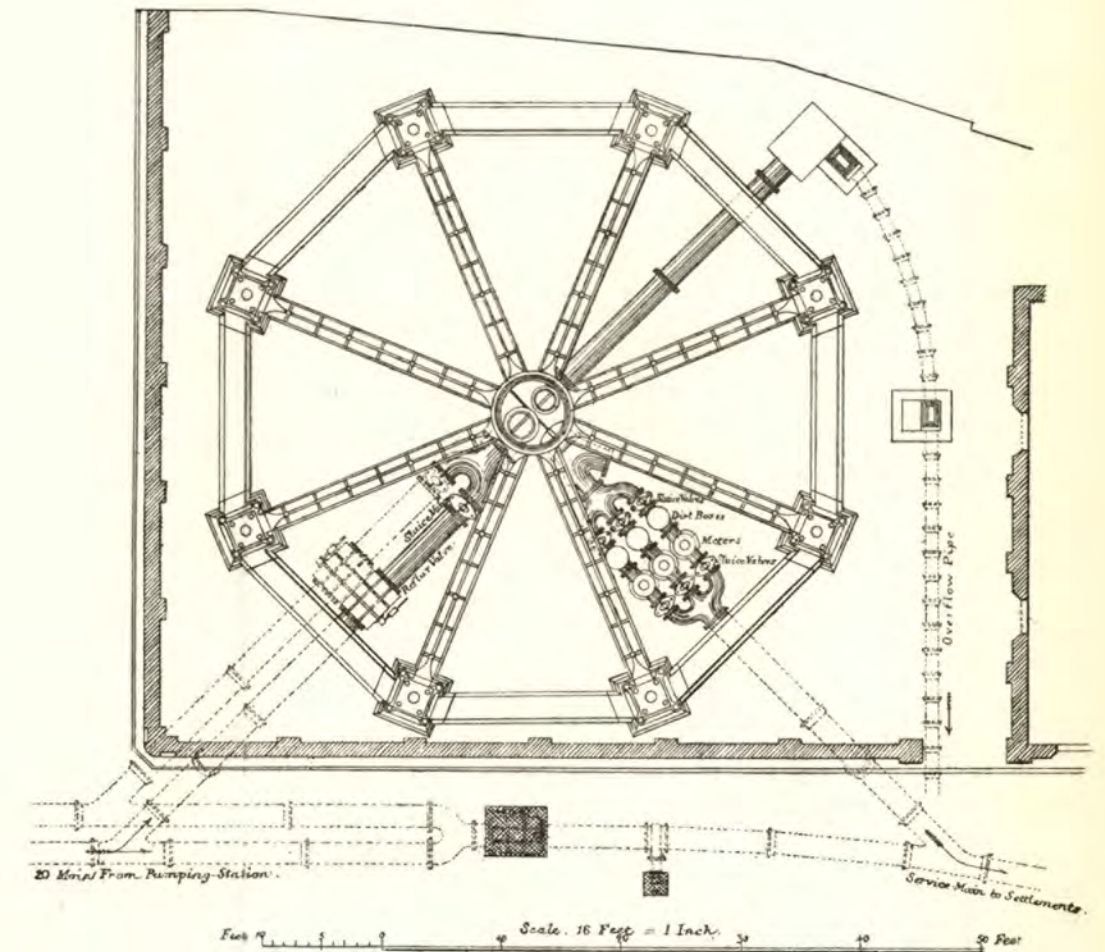
Fig. 145.—Ground Plan of Water Tower at Shanghai.
