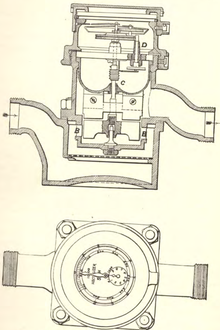
Figs. 233, 234.—Siemens and Halske's patent water meter.
