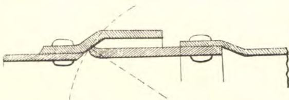
Fig. 219.—The Duncan patent joint for water-pipes.
