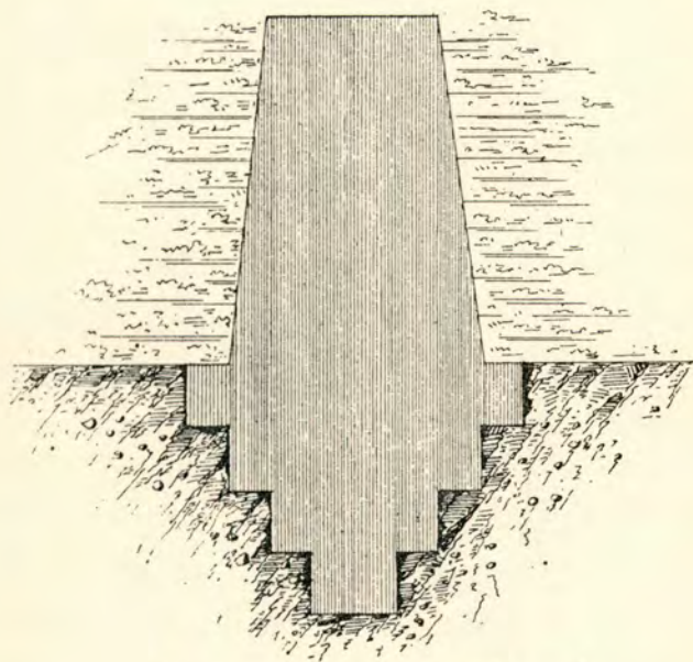
Fig. 19.—Cross-section of puddle trench.
