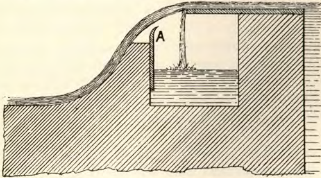
Fig. 47.—Arrangement for directing flow into reservoir.
