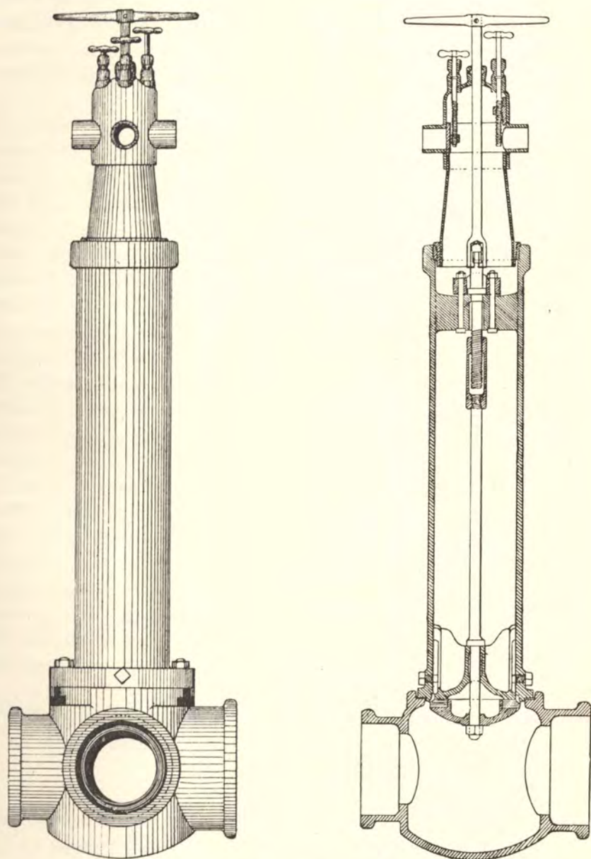
Figs. 196, 197.—Sunk hydrant : American form (Fanning).
