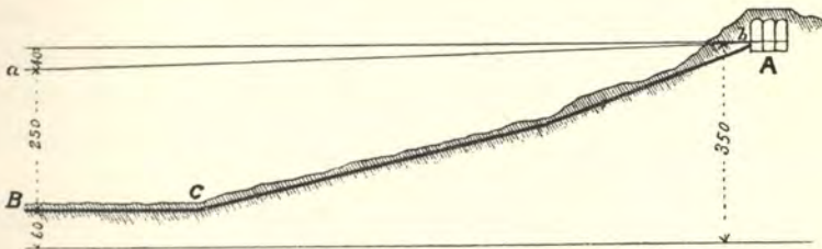
Fig. 174.—Diagram illustrating calculation of hydraulic grade line.
