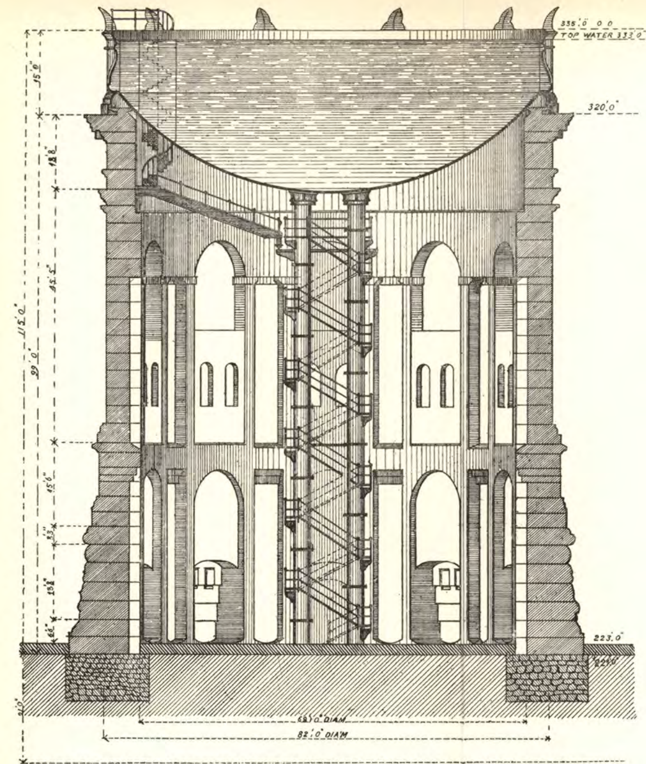
Fig. 143.—Water Tower (in Masonry) at Liverpool.
