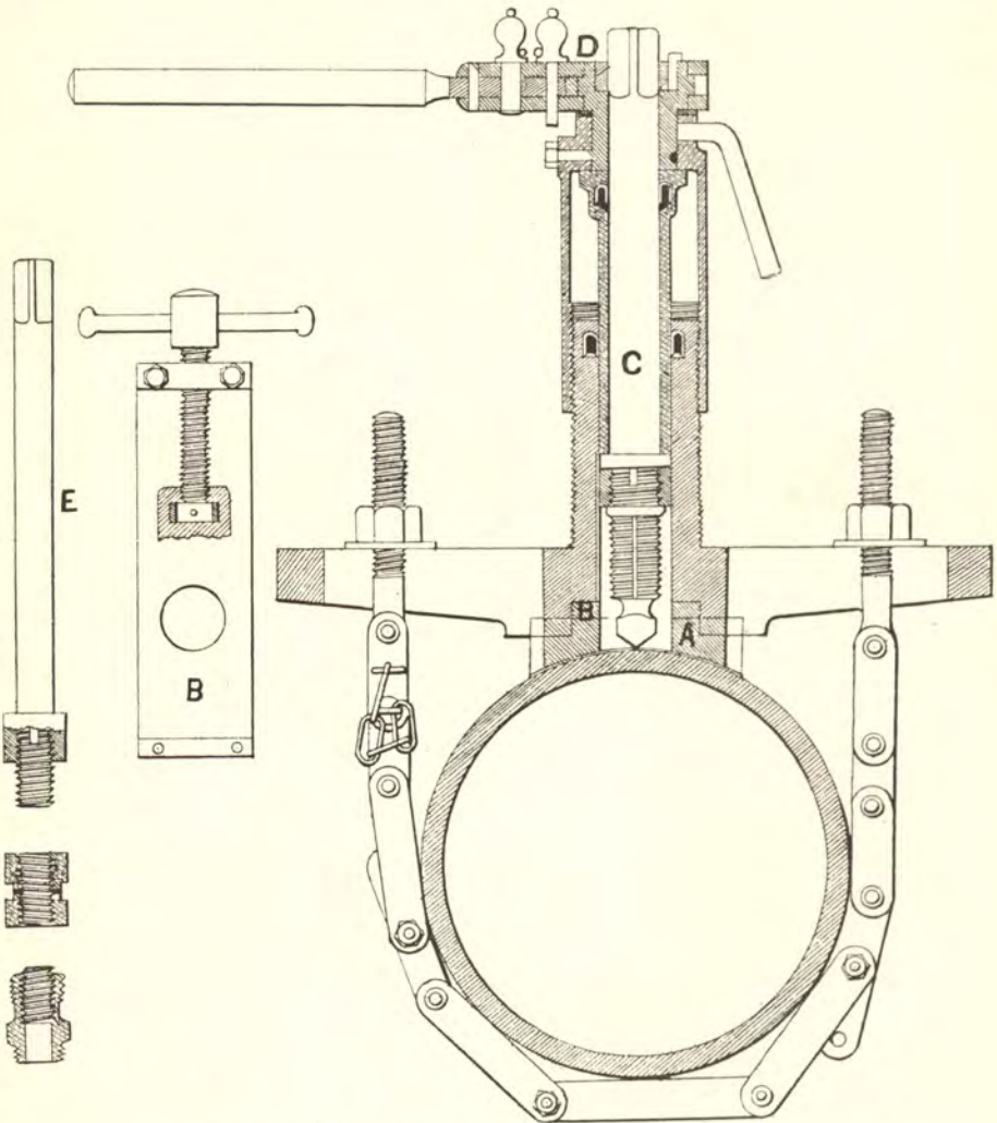
Figs. 250, 251, 252.—Gear for connecting pipes to mains.
