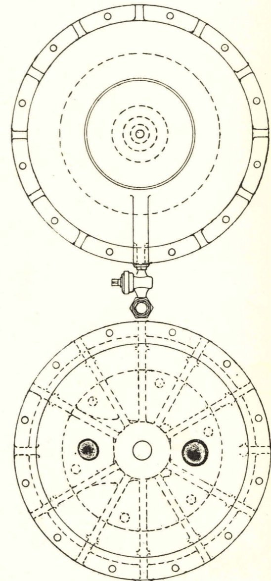
Figs. 37, 38.—Horizontal Sections.
