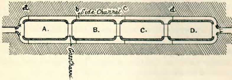
Fig. 57.—Plan of settling tanks.
