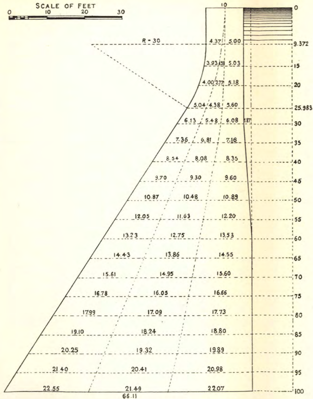
Fig. 52.—Practical Profile No. 2.
