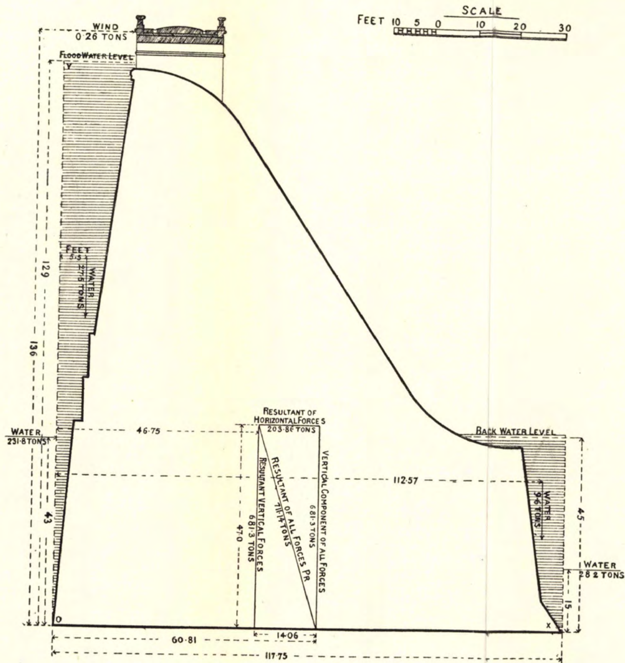
FIG. 55.—SECTION OF VYRNWY DAM (LIVERPOOL WATER SUPPLY).
