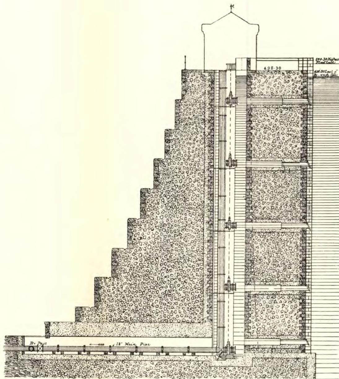
FIG. 56.—TYTAM DAM, HONGKONG : SECTION THROUGH VALVE-WELL.
