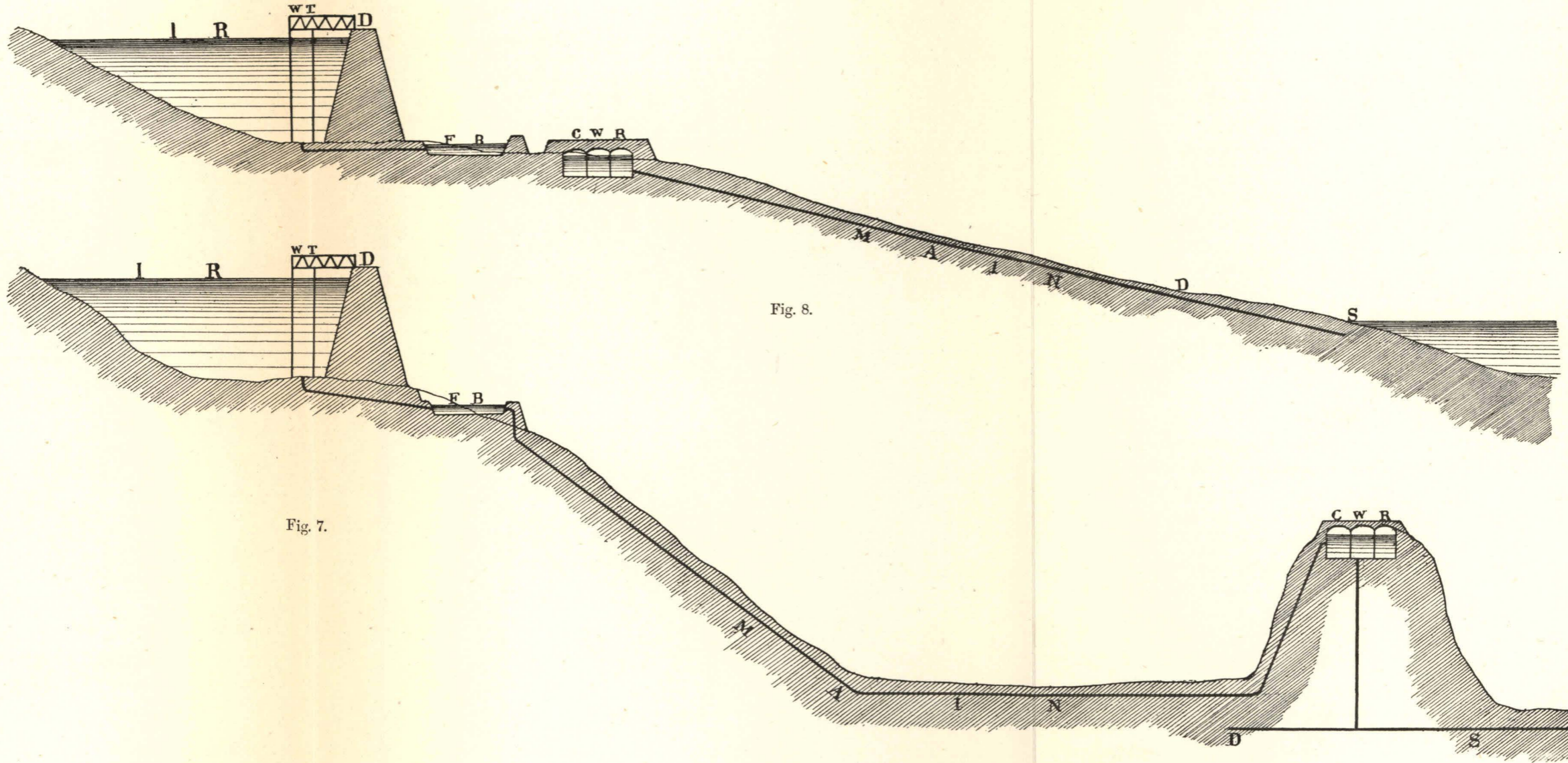
DIAGRAMS ILLUSTRATING GRAVITATION SYSTEMS OF WATERWORKS.
