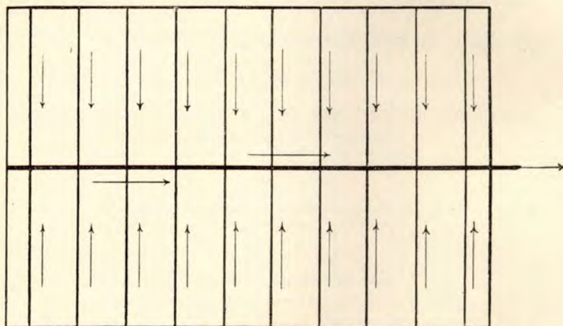
Fig. 92.—Arrangement of drains of filter bed.
