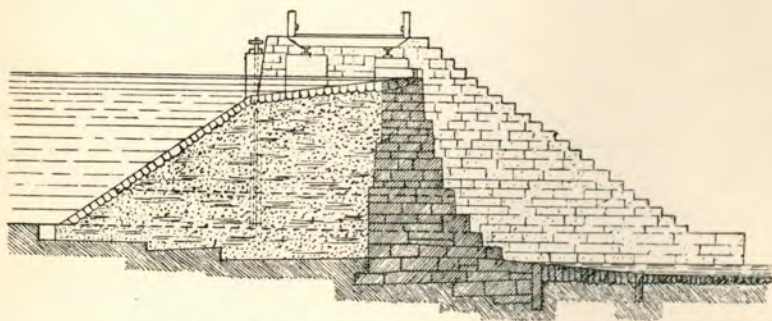
Fig. 45.—Waste weir for water passing over dam (Fanning).
