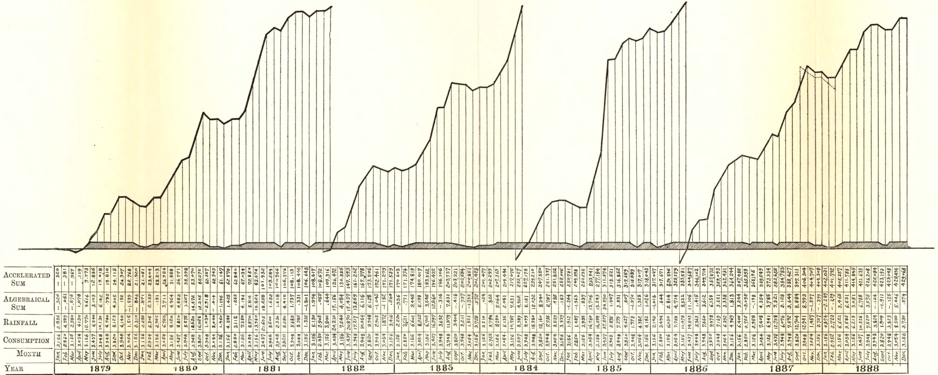
FIG. 5.—DIAGRAM ILLUSTRATING REQUIRED STORAGE CAPACITY (YEARLY RAINFALL).
