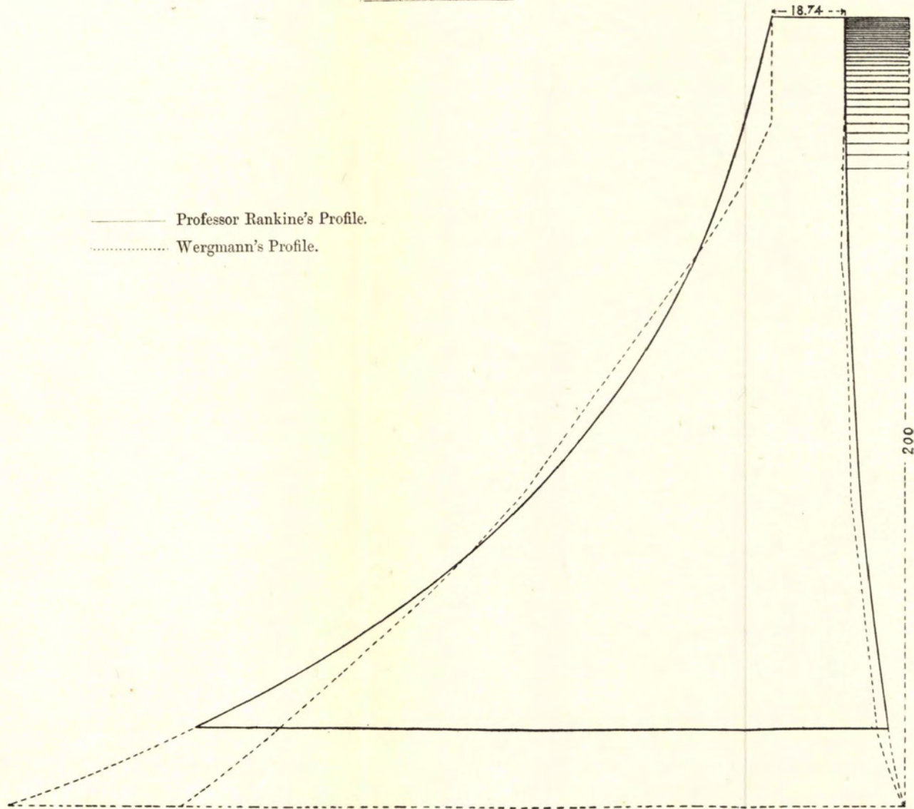
FIG. 49.—MASONRY DAMS: COMPARISON OF RANKINE'S PROFILE WITH THE THEORETICAL PROFILE.
