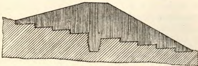
Fig. 48.—Site of dam trenched-out.
