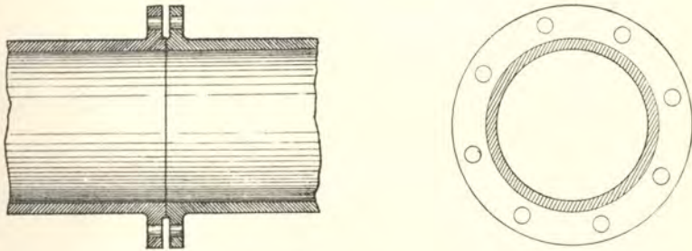
Figs. 198, 199.—Flanged joint for water pipes.
