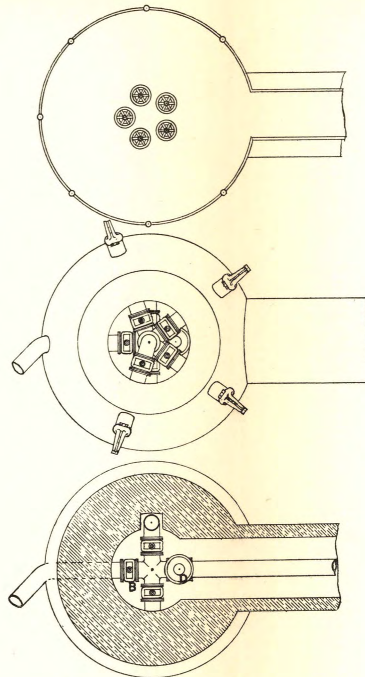
Figs. 32, 33, 34.—Horizontal Sections.
