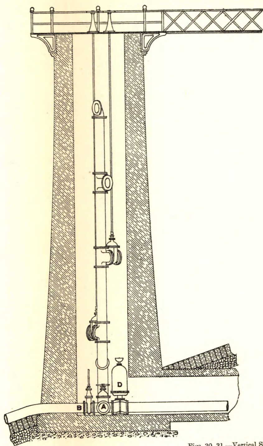
Figs. 30, 31.—Vertical Sections.
