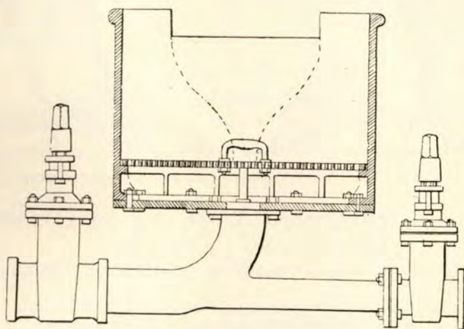
Fig. 122.—Sand-washer.
