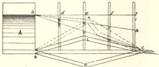
Fig. 173.—Diagram illustrating hydraulic grade line.
