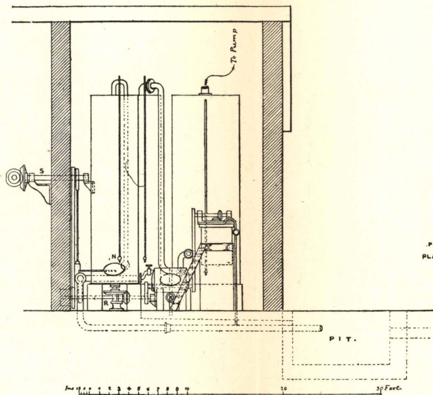
Fig. 132.—Side Elevation.
