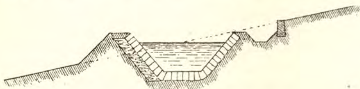
Fig. 151.—Section of open channel on slope.
