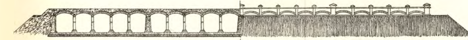
COVERED RESERVOIR: BRICK OR CONCRETE ARCHES ON COLUMNS.
