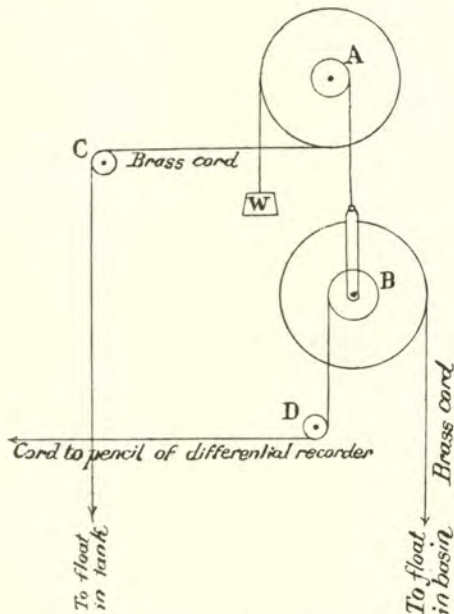
Fig. 222.—Arrangement of pulleys in water meter.
