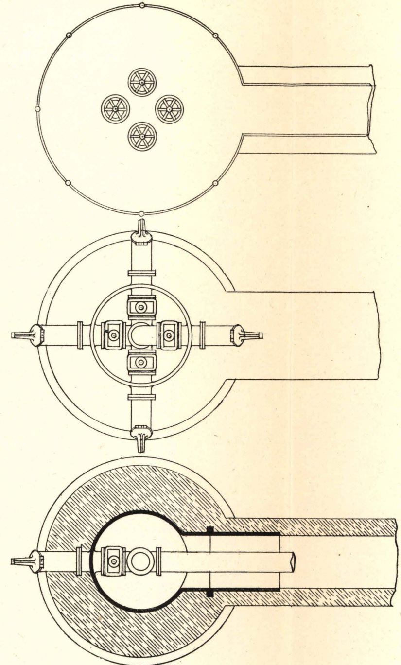
Figs. 41, 42, 43.—Horizontal Sections.
