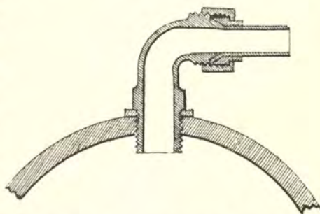
Fig. 249.—Screwed ferrule attached to waterpipe.
