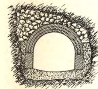
Fig. 168.—Tunnel at Clay or Soft Slips.
