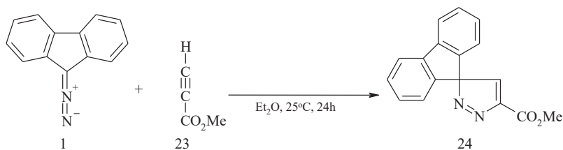
Fig. 10. Synthesis of 3,3-diphenylenepyzolenine carbonic acid-(5)-methyl ester (24)
