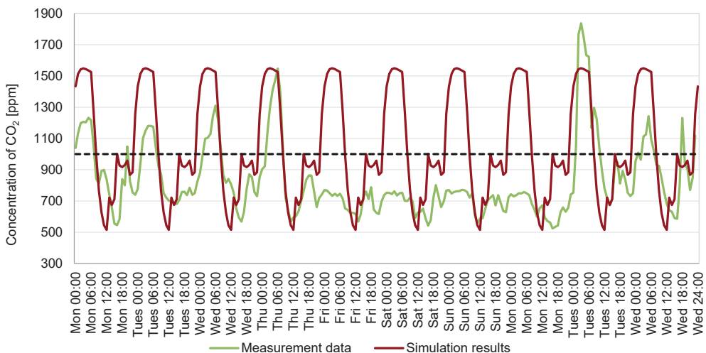
Fig. 6. Carbon dioxide concentration – simulation with the minimal ventilation rate and open door to the walk-in wardrobe; maximum recommended level of 1,000 ppm marked by the dashed line
