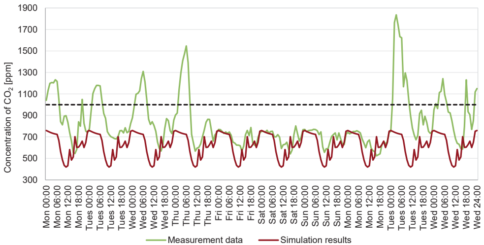
Fig. 11. Carbon dioxide concentration – simulation with the maximum ventilation rate and both doors open; maximum recommended level of 1,000 ppm marked by the dashed line
