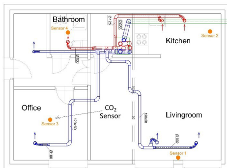
Fig. 4. Ground floor – sensor layout
