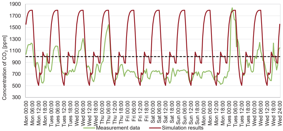
Fig. 7. Carbon dioxide concentration – simulation with the minimal ventilation rate and closed door to the walk-in wardrobe; maximum recommended level of 1,000 ppm marked by the dashed line
