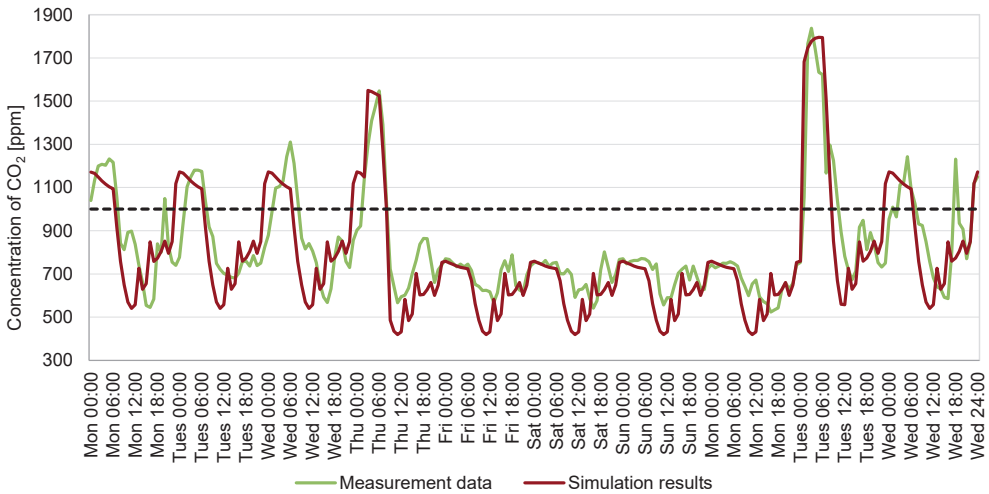
Fig. 12. Carbon dioxide concentration – measurements and the results of simulation with the occupancy schedules and real ventilation rates; maximum recommended level of 1,000 ppm marked by the dashed line
