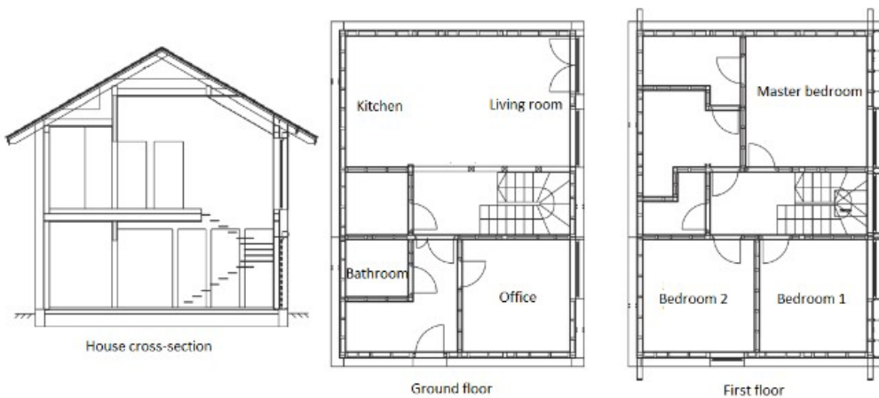
Fig. 1. Test object – plan of the passive house
