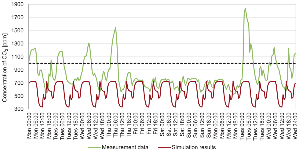
Fig. 10. Carbon dioxide concentration – simulation with the maximum ventilation rate and door to the walk-in wardrobe open; maximum recommended level of 1,000 ppm marked by the dashed line
