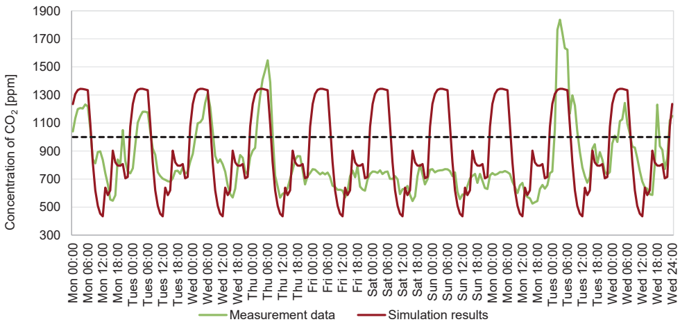
Fig. 8. Carbon dioxide concentration – simulation with the medium ventilation rate and open door to the walk-in wardrobe; maximum recommended level of 1,000 ppm marked by the dashed line
