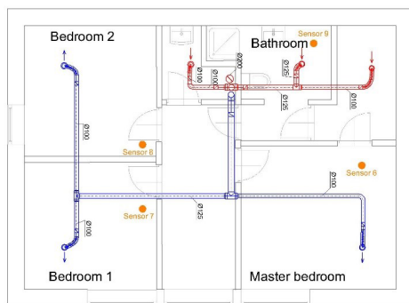
Fig. 3. First floor – sensor layout
