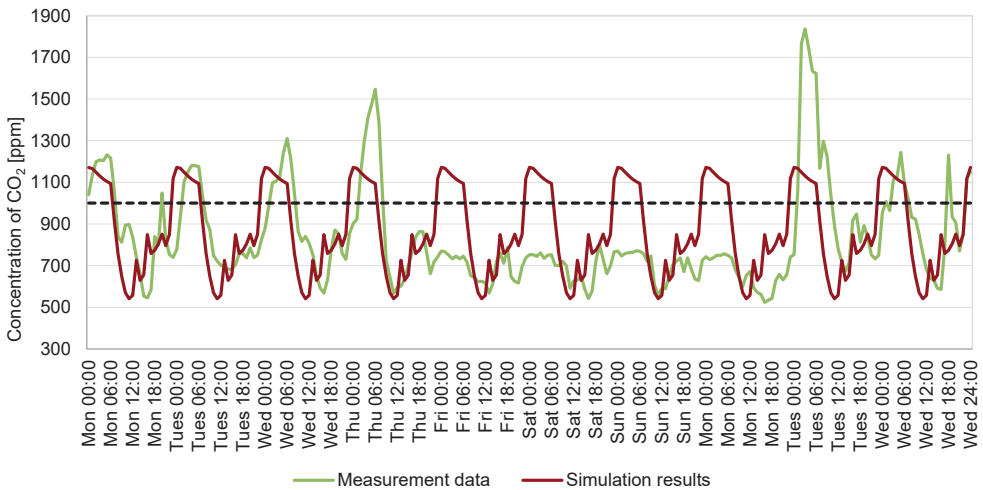
Fig. 9. Carbon dioxide concentration – simulation with the medium ventilation rate and both doors open; maximum recommended level of 1,000 ppm marked by the dashed line
