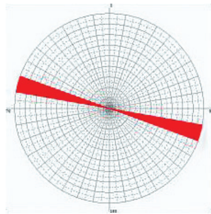
Fig. 3. Direction diagram of the Klodnica fault zone for tremor of 18 April 2015 of seismic energy E=4 \cdot 10^9 J
