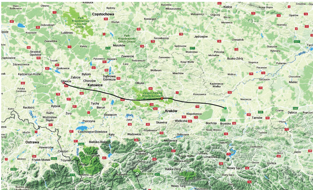
Fig. 4. Trajectory of the balloon predicted according to the wind simulation on 24th of November from [14]
