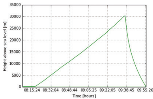
Fig. 7. Height profile for GPS data. Time is given with the respect to GMT
