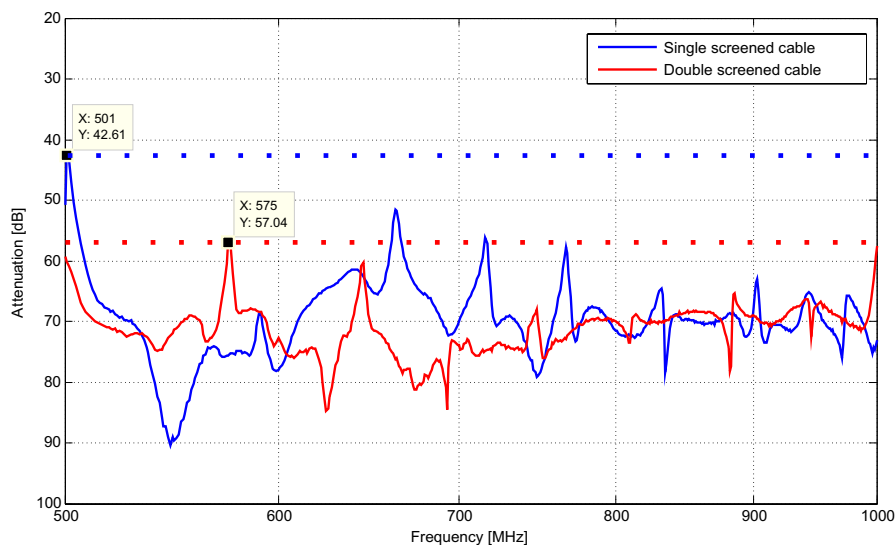
Fig. 6. Screening attenuation in frequency range 500–1000 MHz
