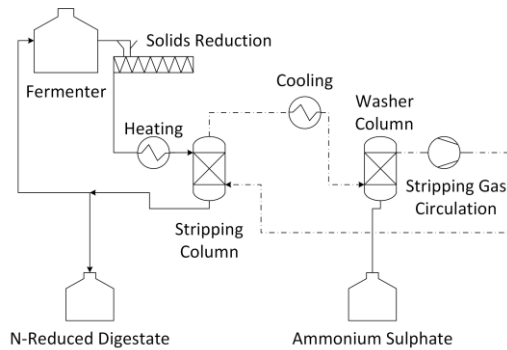
Fig. 9. Stripping process to reduce the ammonium concentration in the digestate and inside the fermenter
