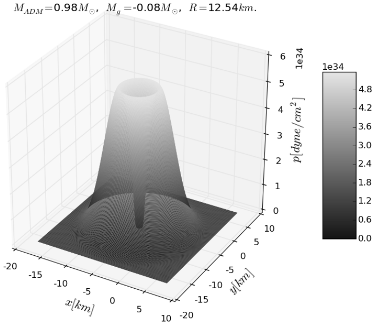
Fig. 1. The pressure profile in 2 + 1 dimensional visualization of a typical nakedly-singular, spherical, polytropic cloud.
