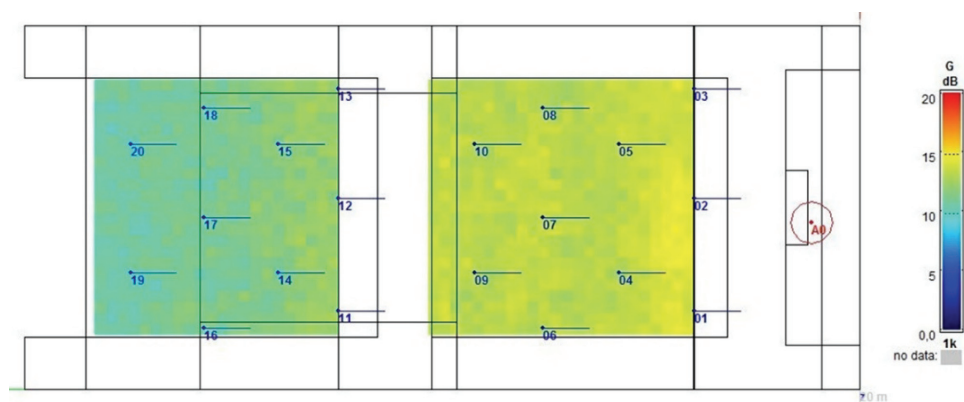
Fig. 21. Map showing the distribution of the sound strength G values in the audience for the A0 sound source location and the octave band with a center frequency of 1 kHz – Variant I
