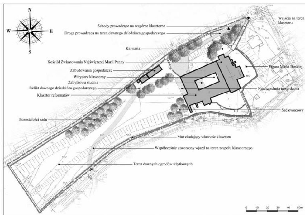
III. 1. Current inventory sketch of the monastery complex in Kazimierz, on the basis of field research as well as land survey and height maps (authors' own study)
