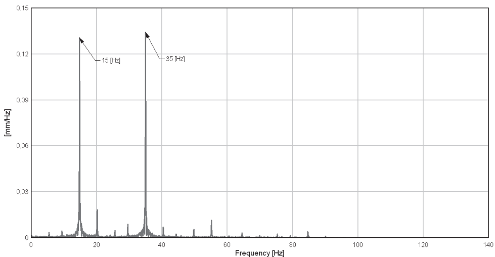
Fig. 11. Spectrum of displacement of the platform for excitation frequency 35 [Hz]
