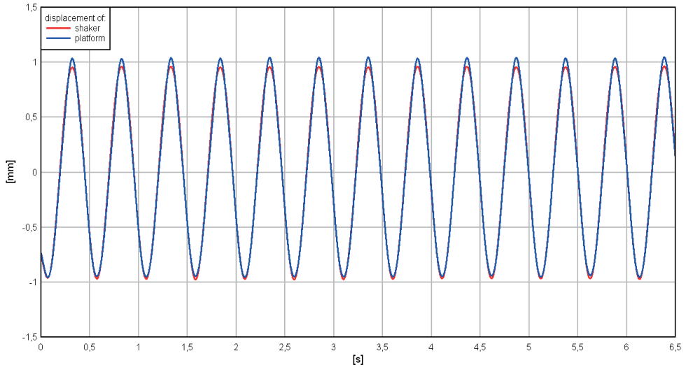
Fig. 8. The time histories of displacements of the shaker and platform for excitation frequency 2 [Hz]
