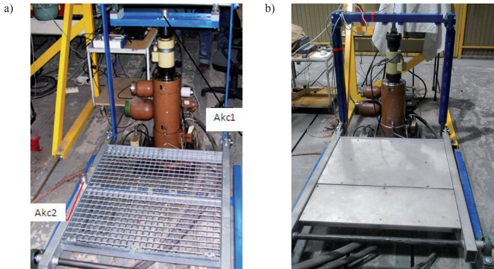
Fig. 1. Primary (a) and final (b) version of the stand
