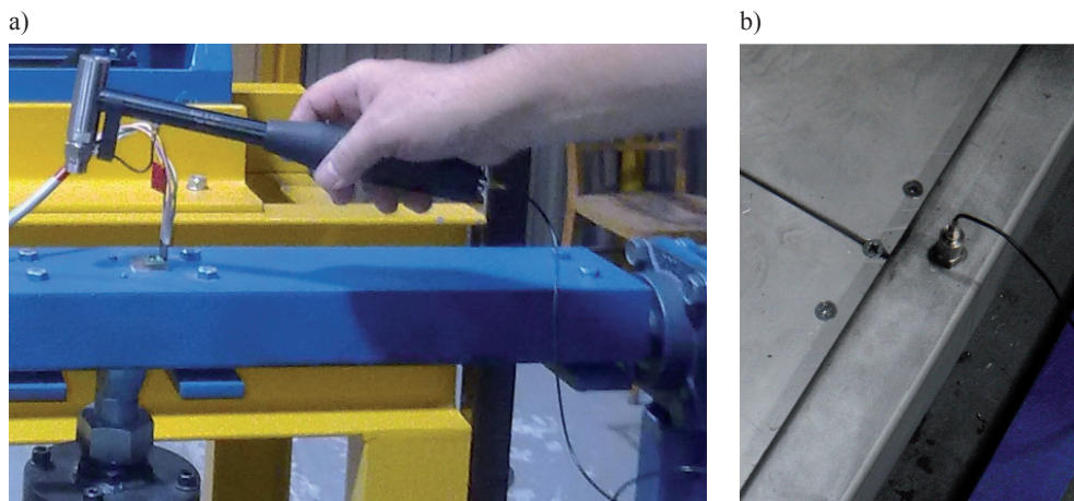
Fig. 4. Impact hammer used as source of excitation (a) and accelerometer used for the response recording of the system (b)
