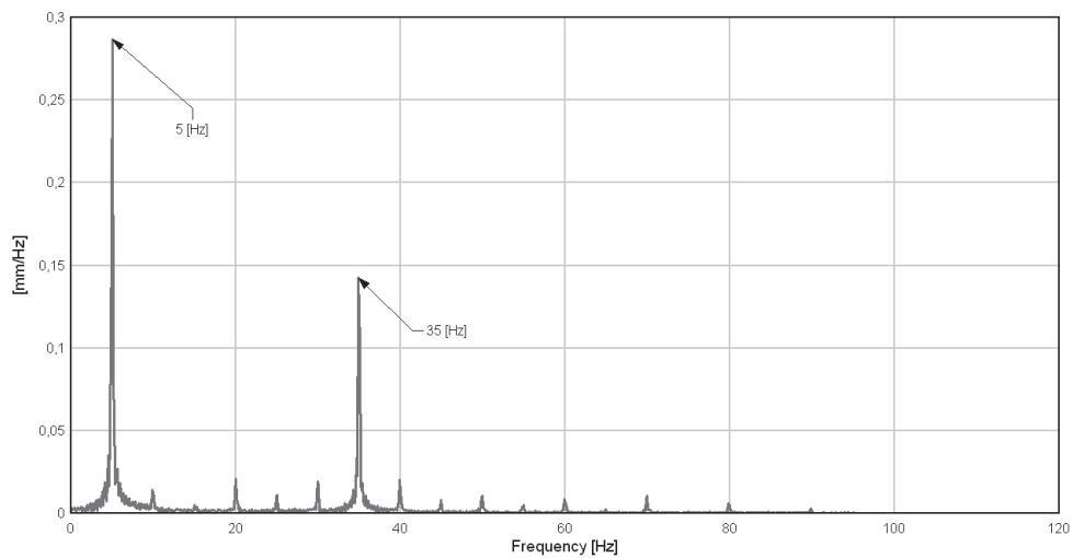
Fig. 10. Spectrum of displacement of the platform for excitation frequency 5 [Hz]
