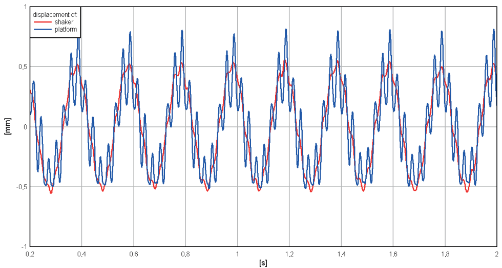
Fig. 9. The time histories of displacements of the shaker and platform for excitation frequency 5 [Hz]
