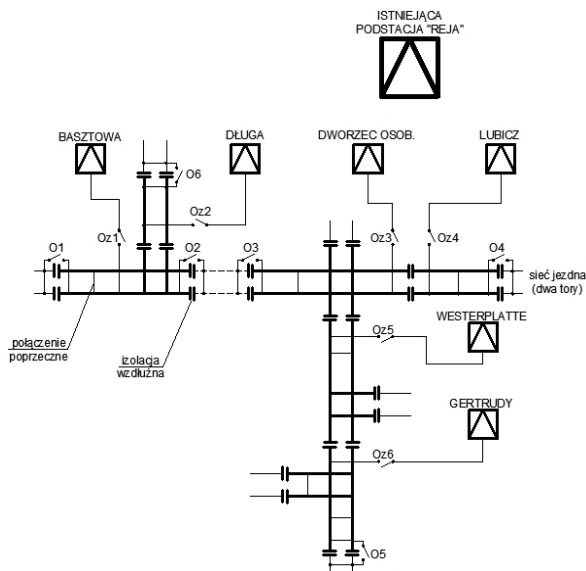
Fig. 2. Connection schematics of a hypothetical tramway system direct current mini-substations with the traction network based on an example of the existing „Reja” substation’s power supply area (Oz1, ..., Oz6 – isolating switches for power supply, O1, ..., O6 – section isolating switches)
