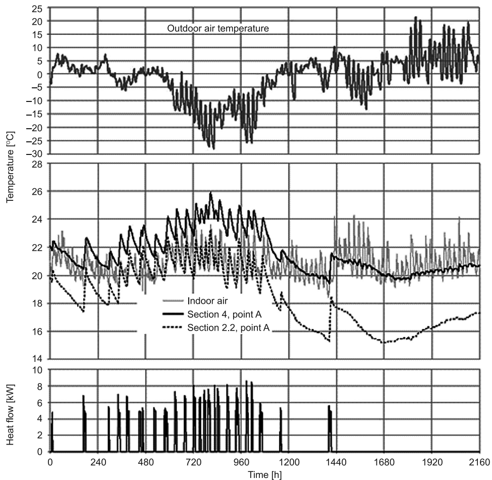
Fig. 5. Pattern of outdoor (top diagram) and indoor temperature, temperature measured at points 4A, 2.2A (lower diagram), and heat supply to floor, 1 st Jan.–30 th March, 2012 (measurement points location shown on Figs. 2, 3)
