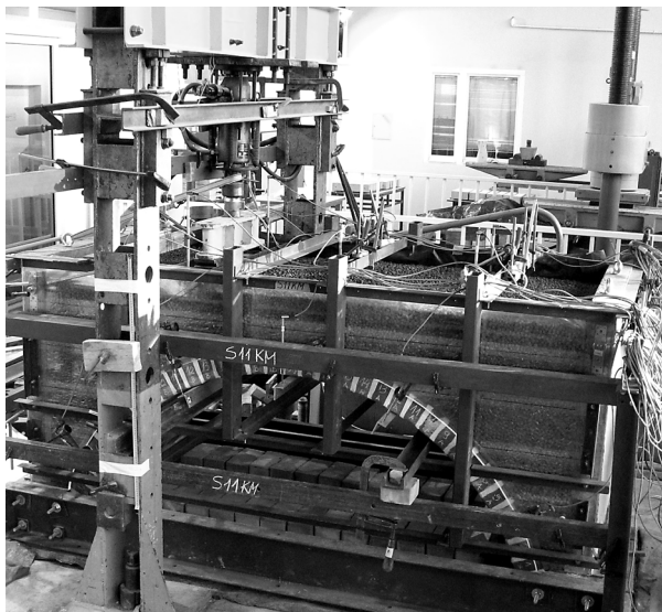
Fig. 2. General arrangement of tested vault – specimen S11KM during the test procedure
