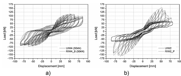
Fig. 9. Hysteresis curves of strengthened walls: (a) strengthening with bolts (higher vertical load level); (b) strengthening with plates (lower vertical load level)
