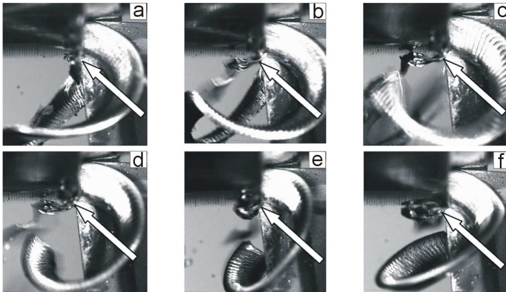
Fig. 5. Sequence of correct chip breaking seen from rake face direction: Inconel 625, v_c=75 m/min, f_n = 0,211 mm/rev, a_p = 1,5 mm, chipformer -23, selected 6 frames out of 23, recording 3100 fps, period between frames a) and f) is 1,65 ms, white arrow points out “additional” chip created by plastic deformation
