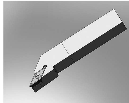
Fig. 2. 3-D model of ISCAR tool and -SM chipformer cross section
