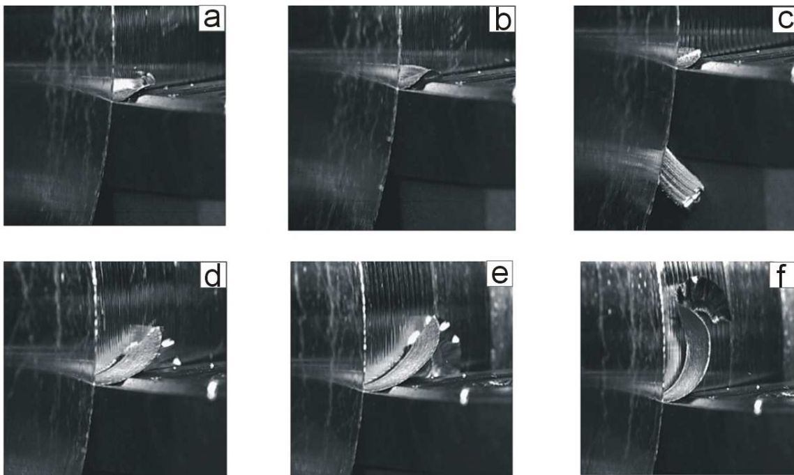
Fig. 9. Example of the lack of control over chip forming in Inconel 718 turning v_c = 50 m/min, a_p = 2,0 mm, f_n = 0,211 mm/rev, chipformer -23, recording rate 1000 fps, period between a) and f) is 79 ms, selection of 6 frames out of 79
