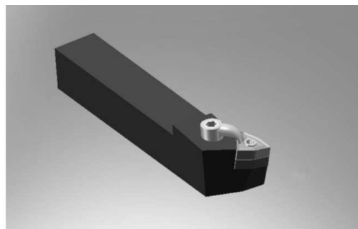
Fig.1. 3-D model of Sandvik Coromant tool and -23 chipformer cross section
