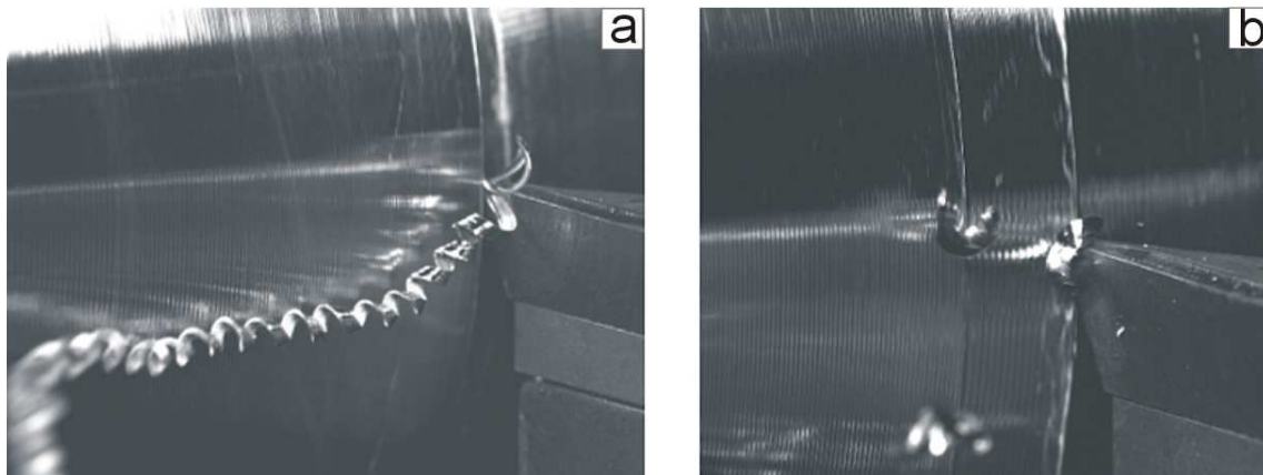
Fig. 7. Example of incorrect chip form, Inconel 625, v_c = 65 m/min, a_p = 0,5 mm, f_n = 0,077 mm/rev, and correct form for the same cutting speed and depth of cut but for the feed f_n = 0,249 mm/rev, recording 1000 fps, a) incorrect chip form, b) correct chip form,
