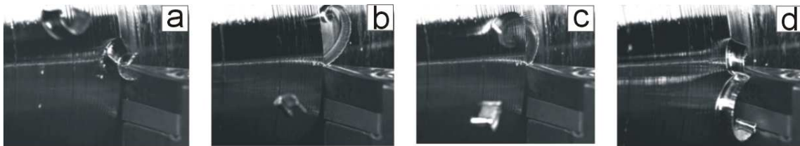
Fig. 8. Two kinds of chip breaking way in one cut, Inconel 625 v_c = 65 m/min, a_p = 2,5 mm, f_n = 0,153 mm/rev, chipformer -SM, recording 1000 fps, a) end of breaking cycle, b) chip hits the raw surface of the workpiece and bends back, c) suddenly chip slips to the left, d) breaking process ends by hitting flank surface of the insert
