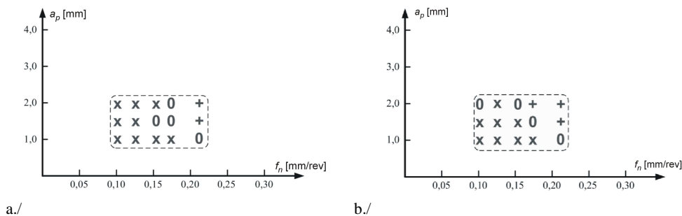
Fig. 10. Useful areas of chipformer -23 application in turning: a) Inconel 718 and b) Inconel 625
