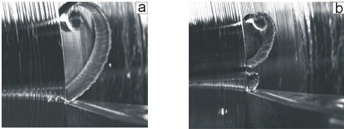
Fig. 6. Chipbreaking by hitting workpiece raw surface: Inconel 625 v_c = 65 m/min, a_p = 2,5 mm, f_n = 0,153 mm/rev, chipformer –SM; a) chip hits raw surface of the workpiece and bends back, b) bending strength is exceeded and the chip splits
