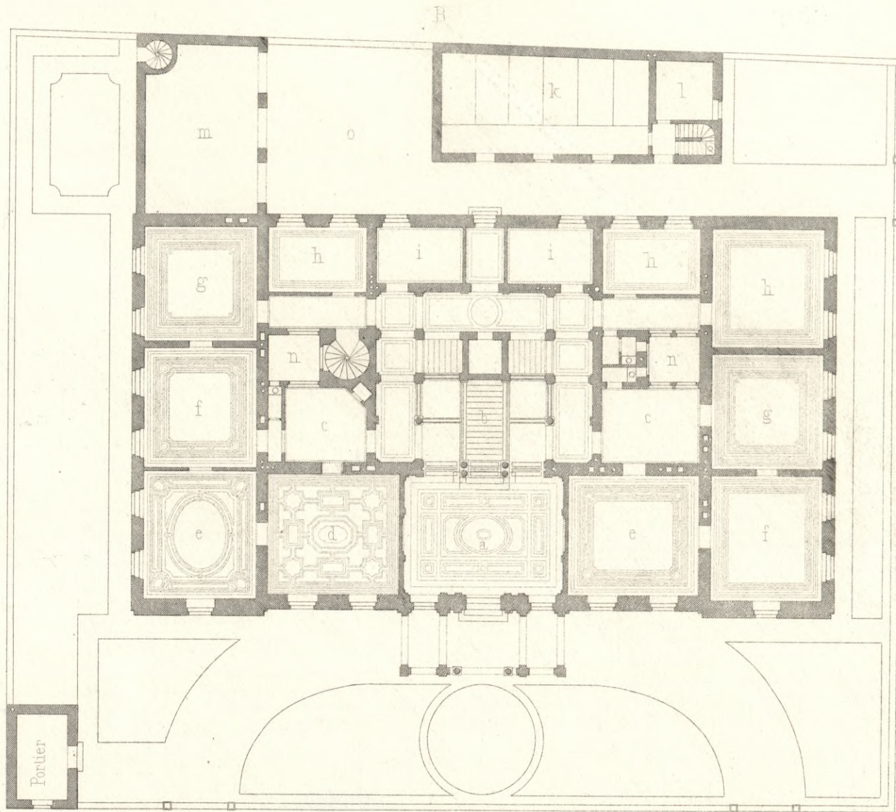
B. ERDGESCHOSS.
