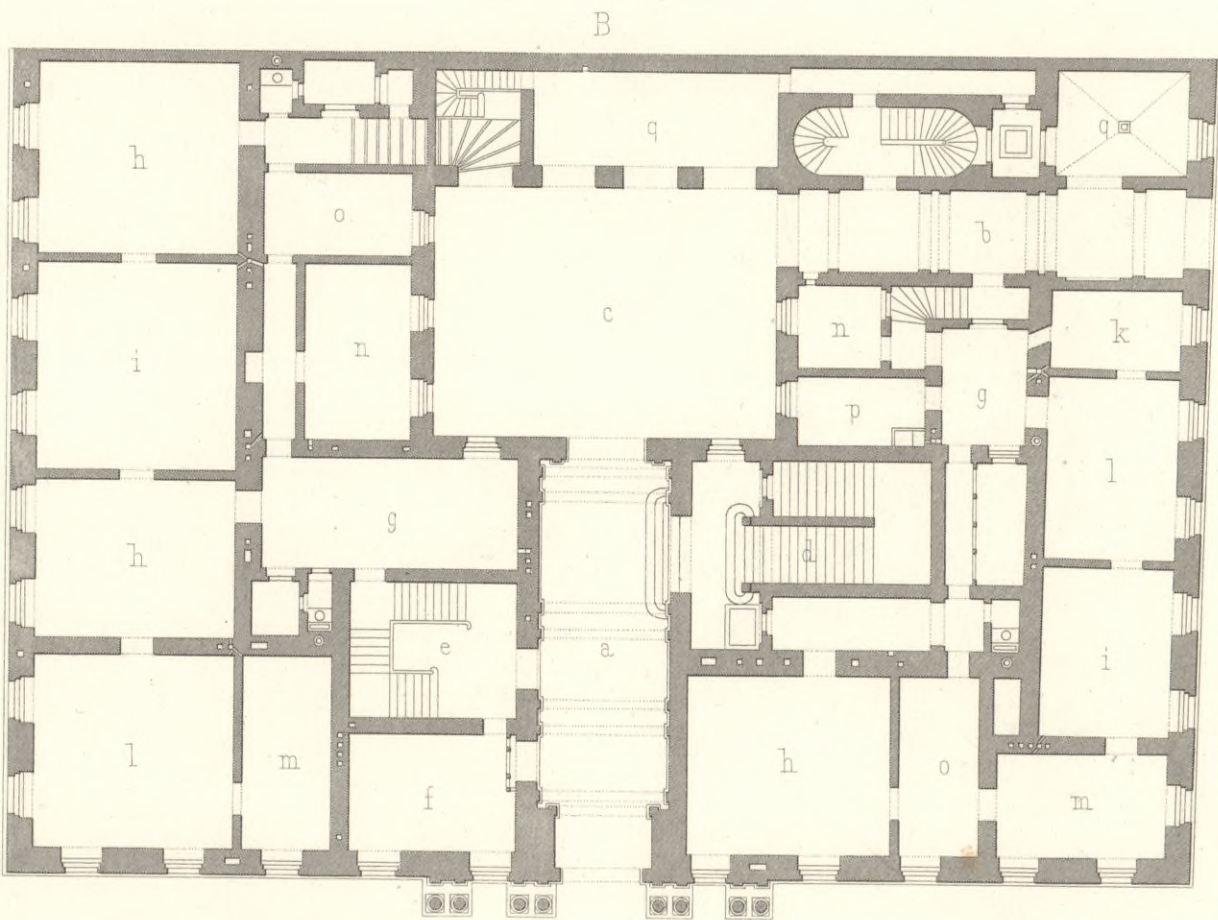
B. ERDGESCHOSS.
