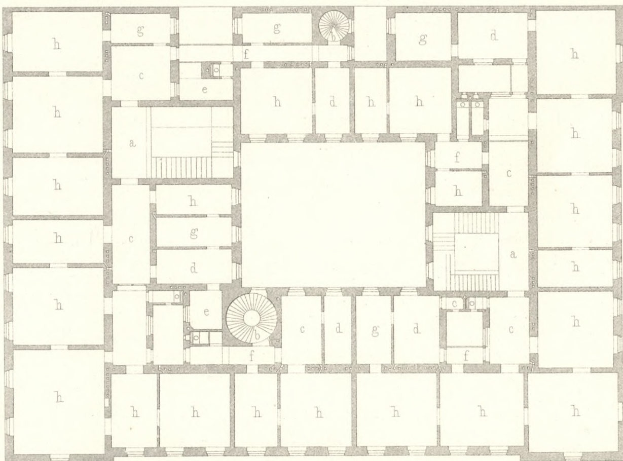
II. u. III. STOCK.
