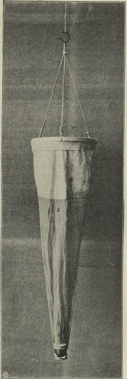
Abb. 79. Qualitatives Planktonnetz.
