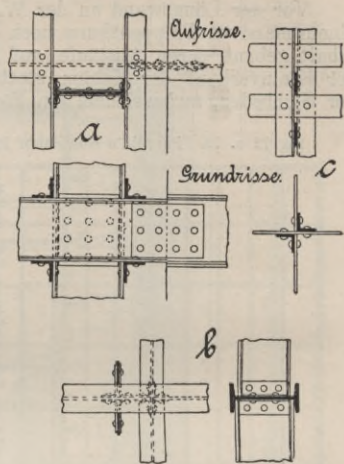
Fig. 74–76. Possehl's Kohlenhof in Hamburg-Altona.
