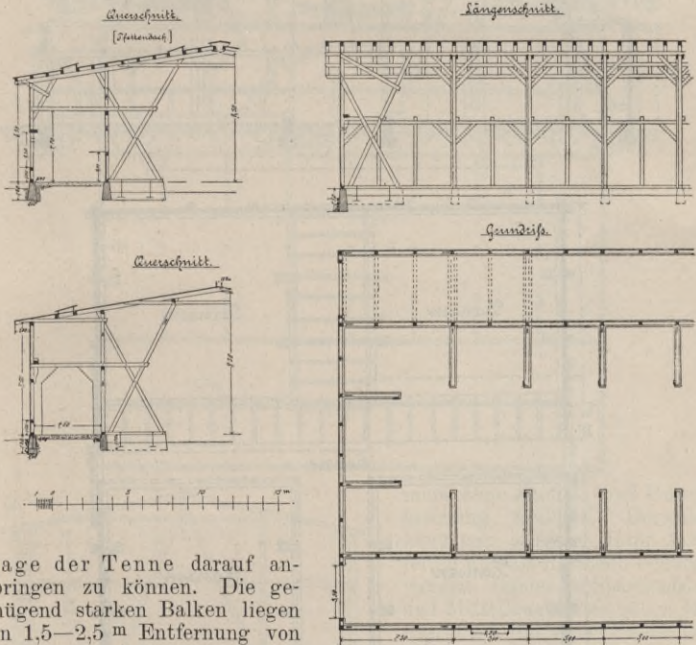
Fig. 104—107. Scheune in Tessin i. M. Arch. Wagner.
