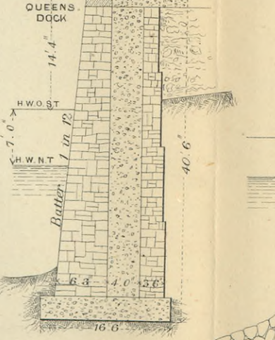
Fig. 16. WHITEHAVEN. EAST QUAY.
