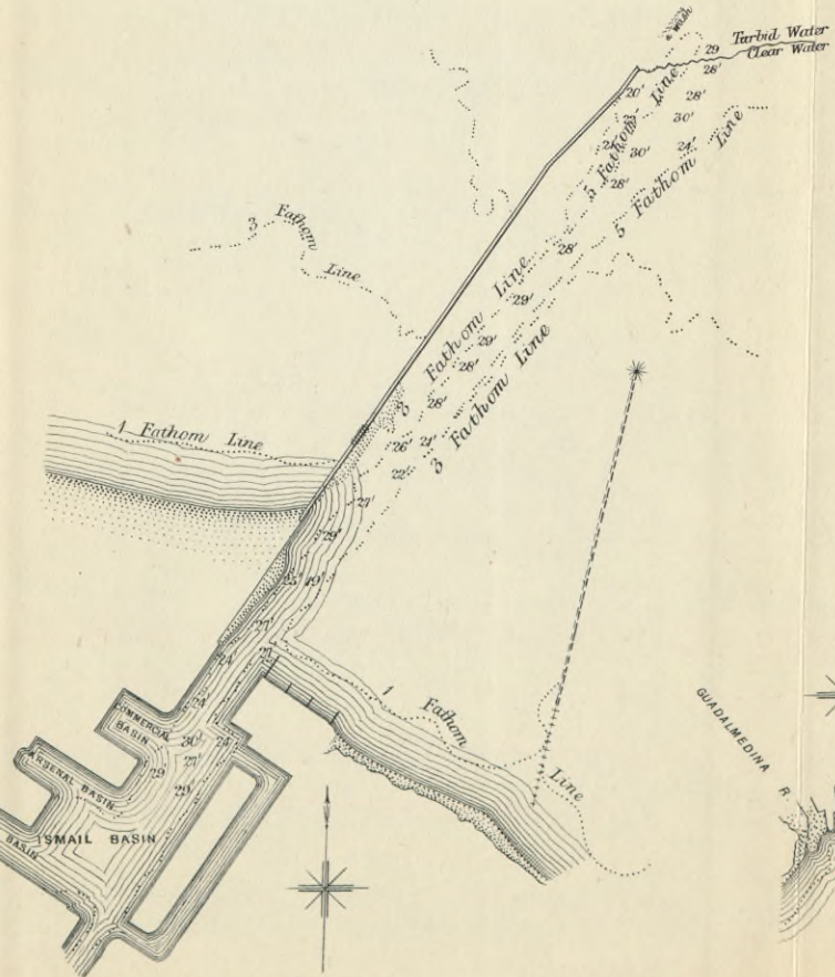
Fig. 7. PORT SAID HARBOUR.
