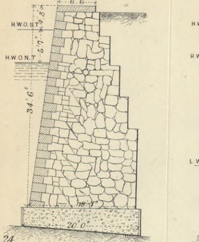
Fig. 24. HAVRE 9TH DOCK.
