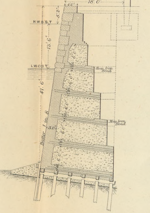
Fig. 9. PORTSMOUTH. TIDAL BASIN EXTENSION.
