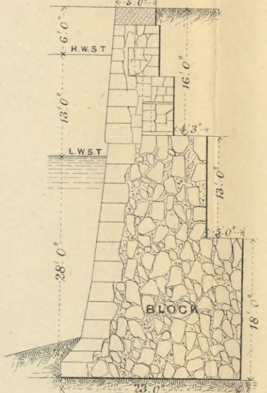
Fig. 16. WHITEHAVEN. EAST QUAY.
