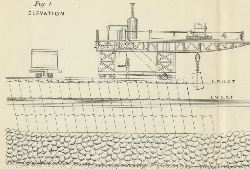
TITAN MANORA BREAKWATER.
