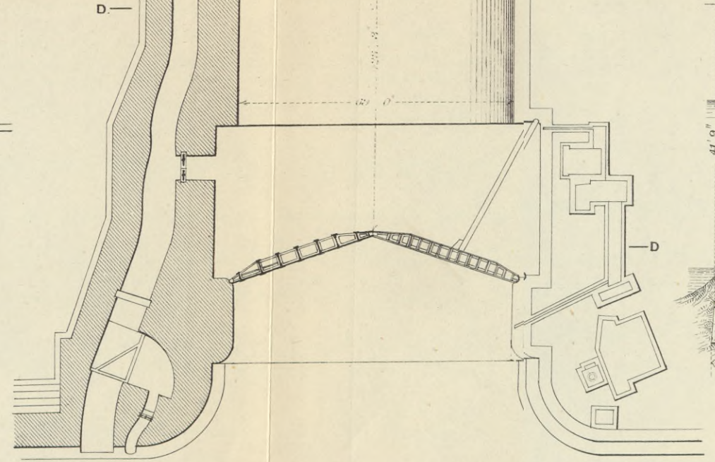
Fig. 9. Nº 1. DOCK DUNKIRK OUTER END OF LOCK
