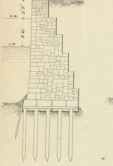
Fig. 17. BELFAST. SPENCER DOCK.
