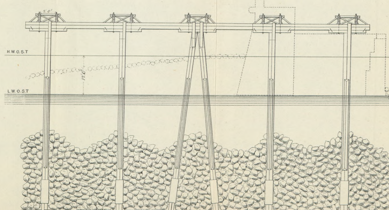
Fig. 10. CROSS SECTION.
