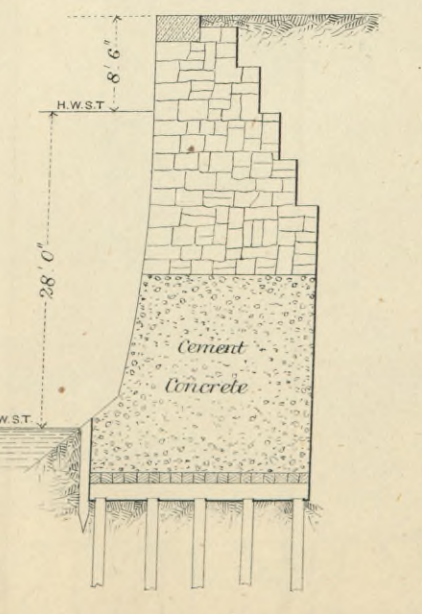
Fig. 14. BARROW. WALL OUTSIDE ENTRANCE.
