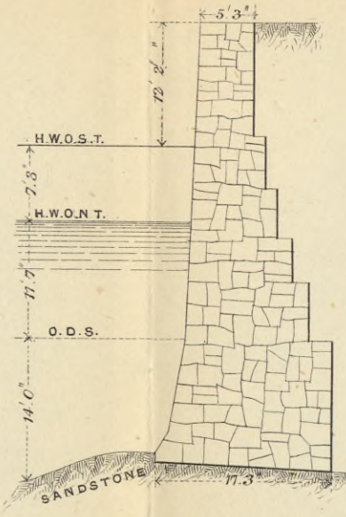
Fig. 3. WEST INDIA DOCKS.
