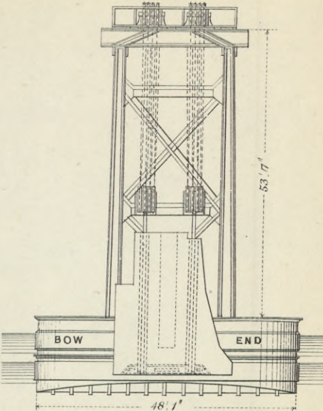
Fig. 12. END ELEVATION.
