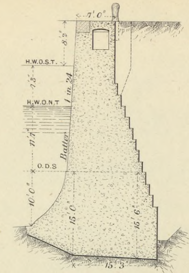
Fig. 2. NEW DOCK NORTH END.
