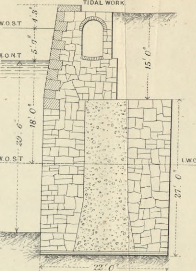
HAYRE. 9TH DOCK TIDAL WORK.
