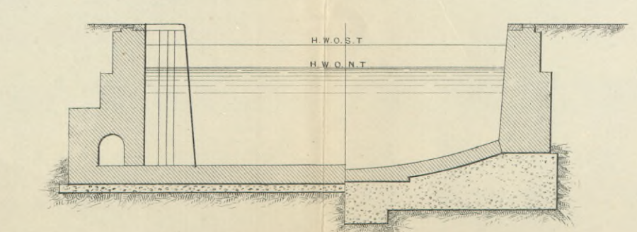
Fig. 6. SECTION ON B B
