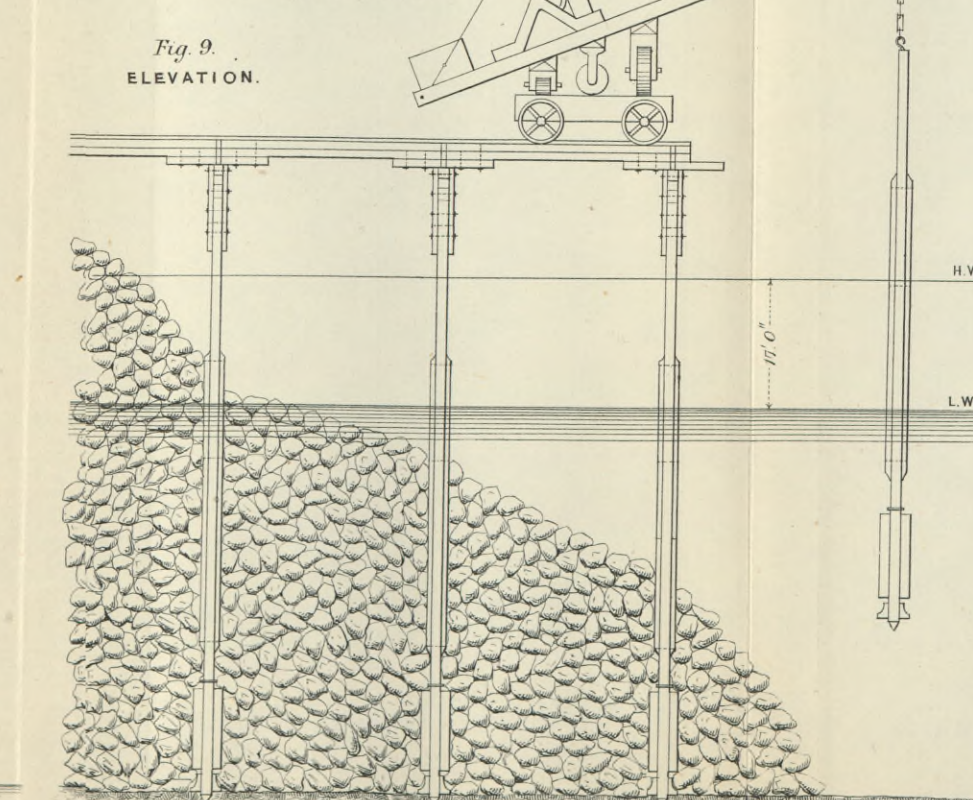
STAGING HOLYHEAD HARBOUR.
