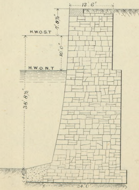
Fig. 4. BUTE DOCKS, CARDIFF ROATH BASIN
