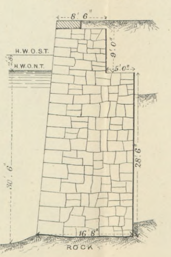
Fig. 12. QUEENSTOWN HAULBOWLINE ISLAND
