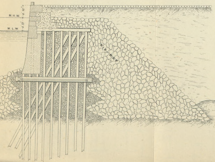
Fig. 18. NEW YORK. NORTH RIVER.
