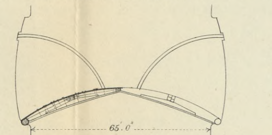
Fig. 3. BRISTOL. INNER GATES, ENTRANCE LOCK.
