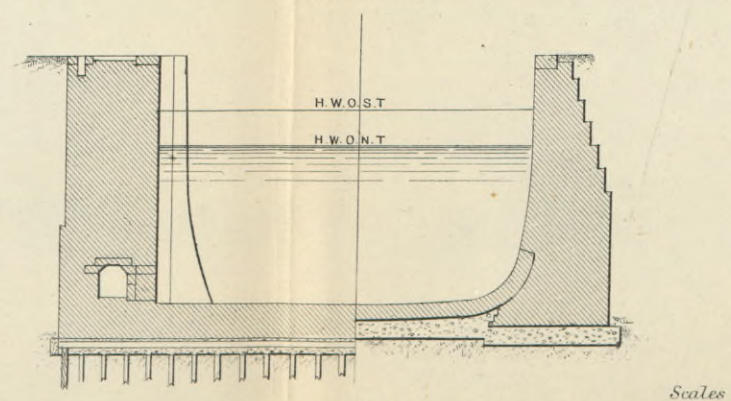
Fig. 8. SECTION ON C.C.
