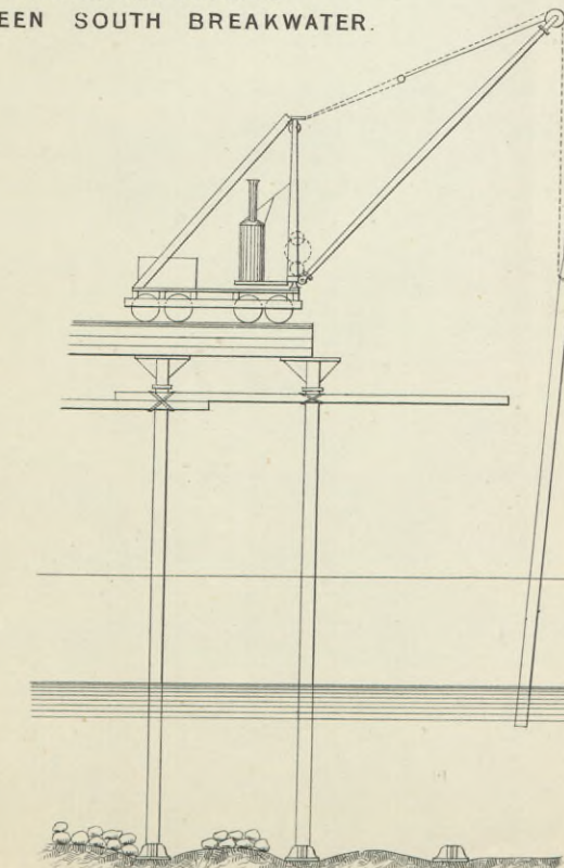
CRANES AND STAGING ABERDEEN SOUTH BREAKWATER.
