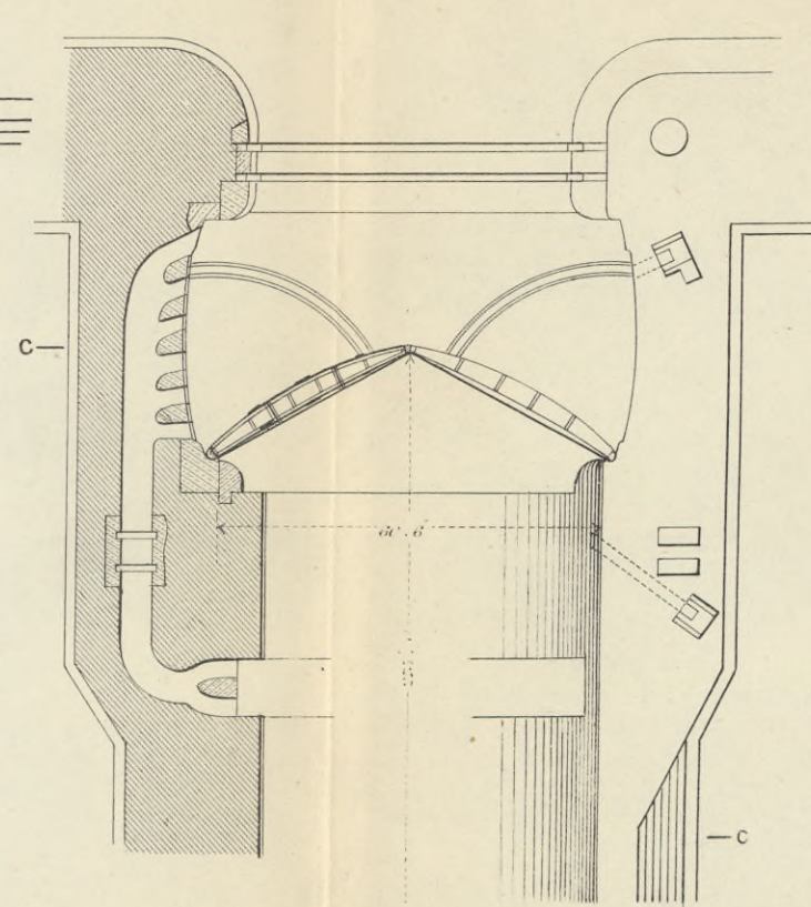
Fig. 8. SECTION ON C.C.
