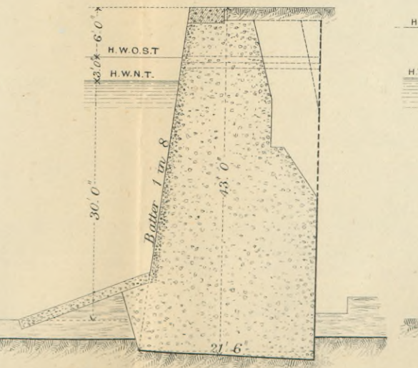
Fig. 10. CHATHAM. FITTING OUT BASIN.
