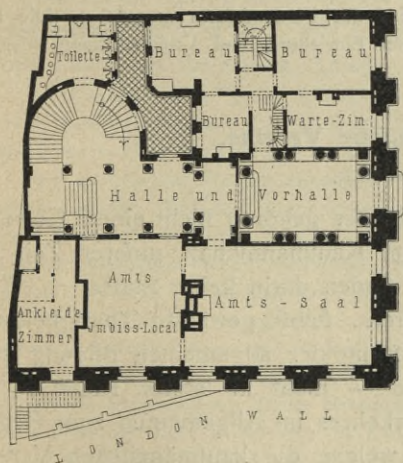
Fig. 289. Erdgefchoff.
