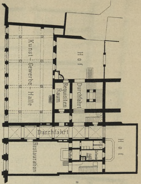
Fig. 298. Erdgeschoss.
