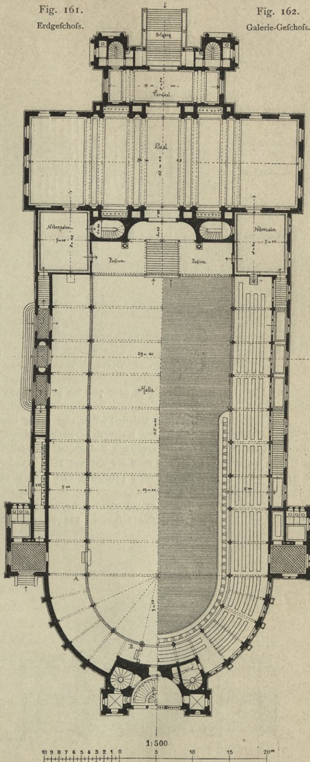
Festhalle in Karlsruhe.
