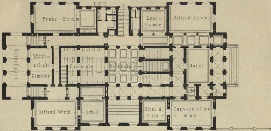
Fig. 258. Erdgeschoss.
