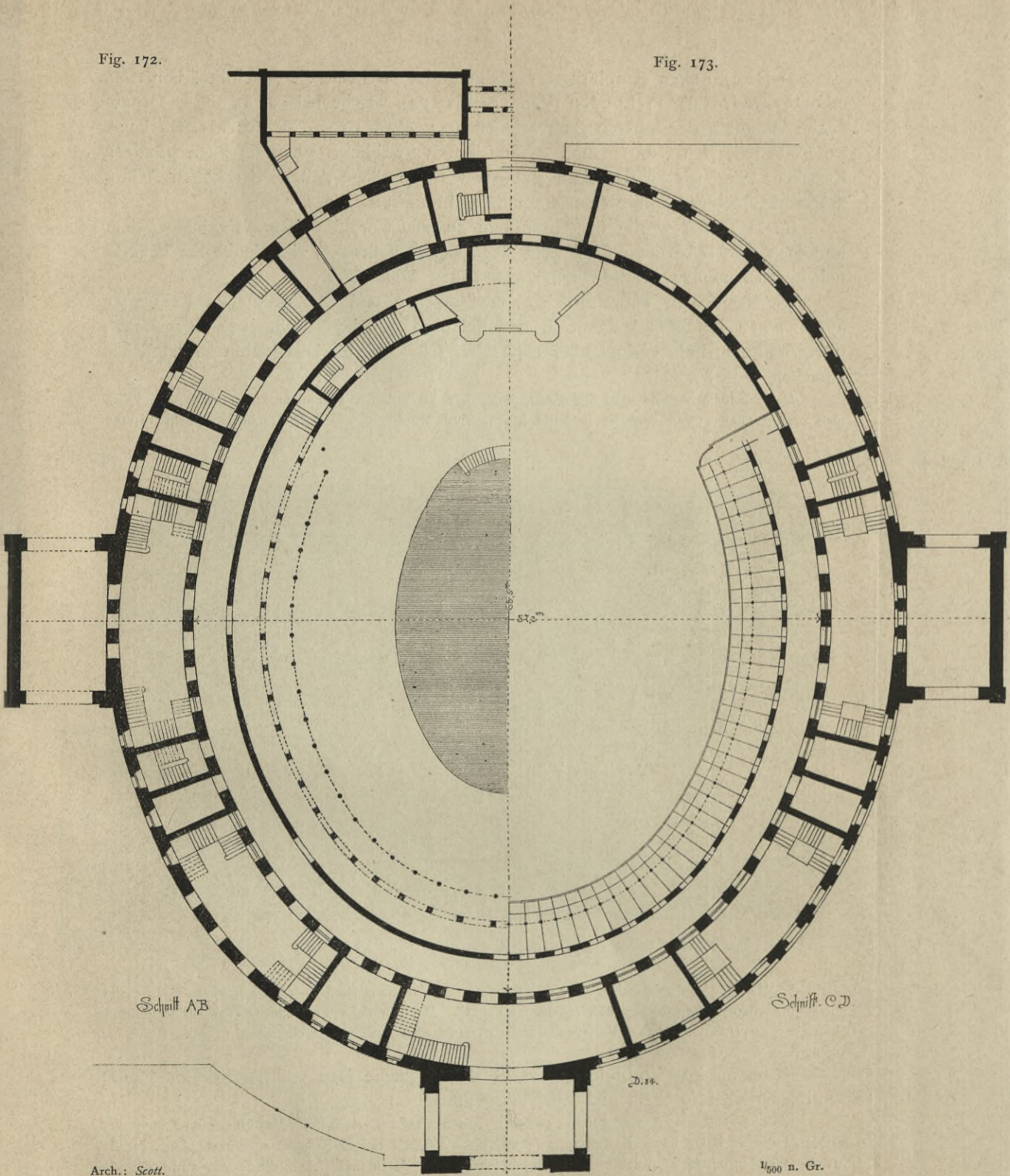
Albert-Halle in London.
