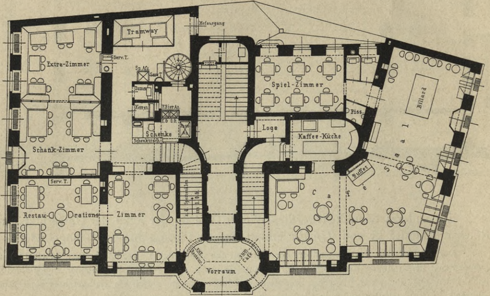
Erdgeschoss.
