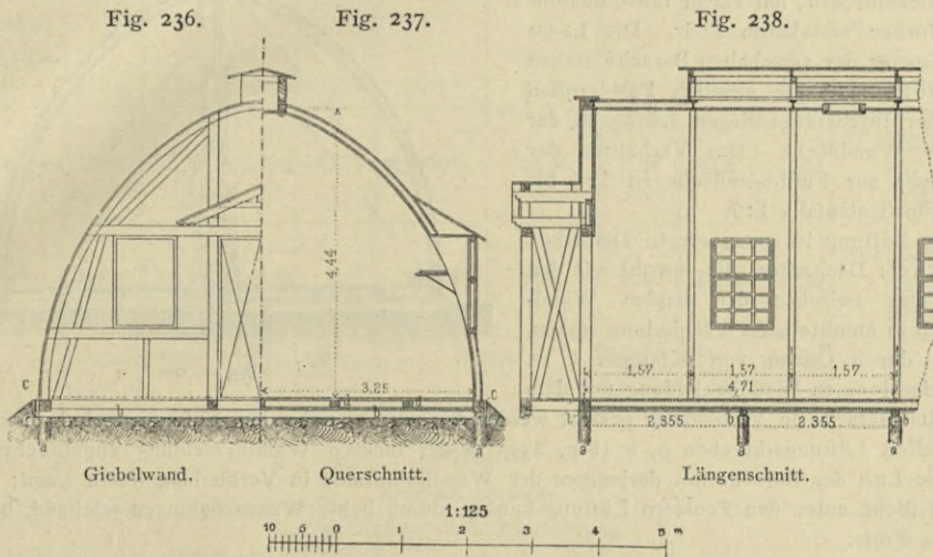
Lagerbaracke. — System Völckner.
