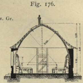
Tolle's Lagerpavillon.
