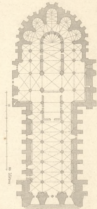
Cathedrale zu Rheims. Grundriss. 5
