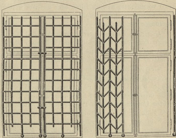
Born's Patent-Gitter 30) .
