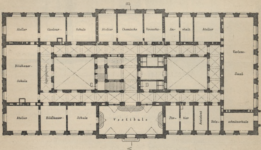
Erdgeschoss.
