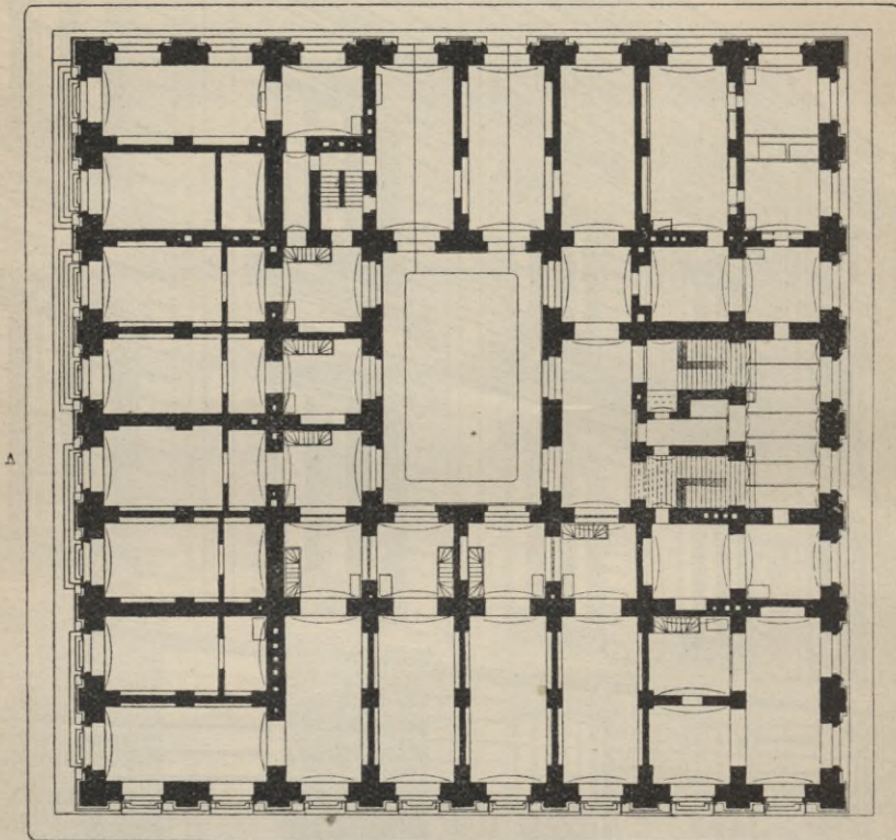
Erdgeschoss.
