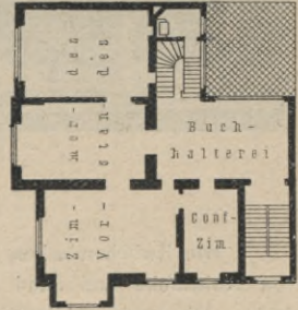
II. Obergeschoss.
