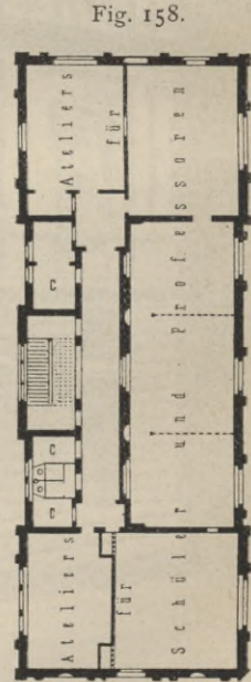
II. Obergeschoss.
