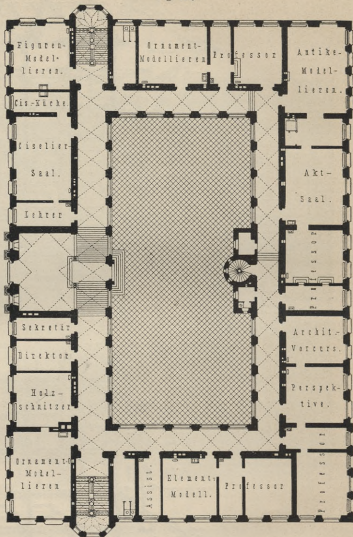
Erdgeschoss.
