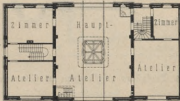
Erdgeschoss.
