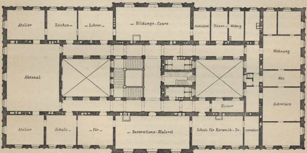
II. Obergeſchoß.
