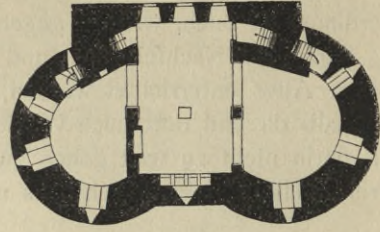
II. Obergeschoss.
