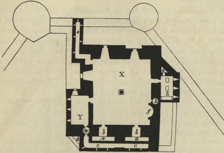
III. Obergeschofs.
