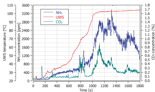
Figure 2. Results of \text{NH}_3 and \text{CO}_2 concentration measured over urea–water solution heat-up.
