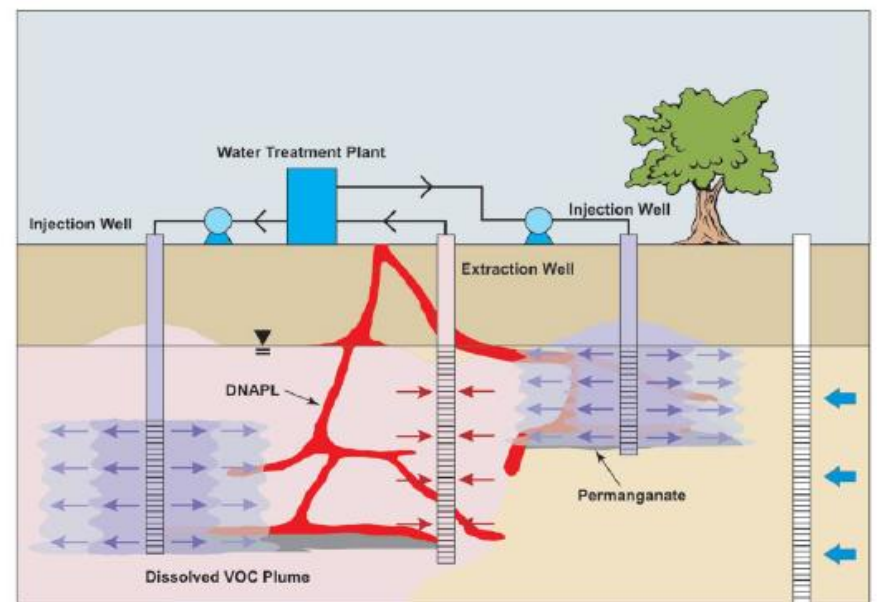
Figure 7. In-situ permanganate oxidation involving the recirculation method. Injection and extraction wells are used to deliver and recover the oxidant solution. Above-ground treatment is required to remove particulate matter (i.e. MnO_2(s) , sand, silicates) and possibly COCs/ VOCs, and to re-amend the ground water with permanganate before re-injection.
