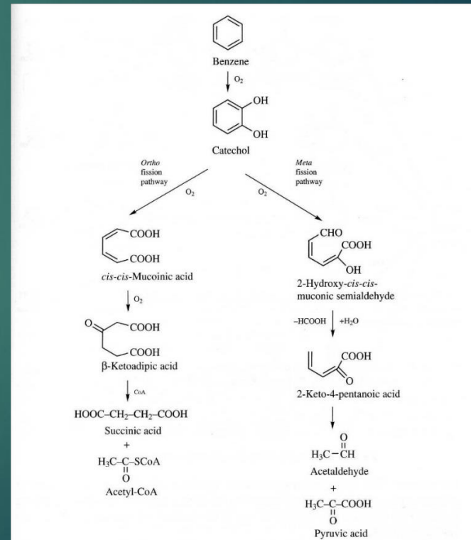
Figure 3.19. Microbial degradation of aromatic compounds by the ortho and meta fission pathways, as illustrated for benzene.
