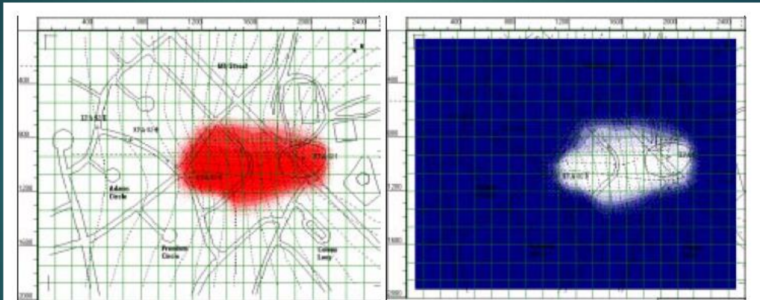
Figure 2.9 Plume Migration for BTEX and Oxygen After a 1 Year Simulation.
