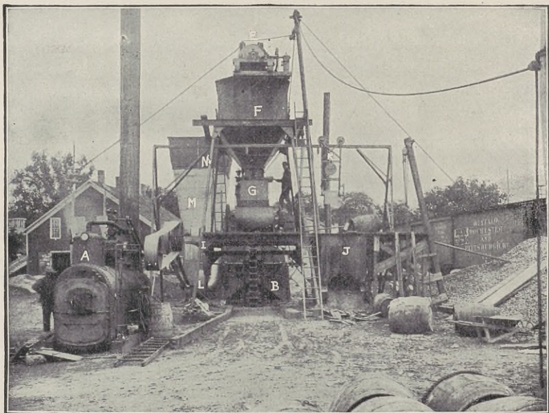
END VIEW.
