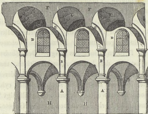
St. Philibert, Tournus.
