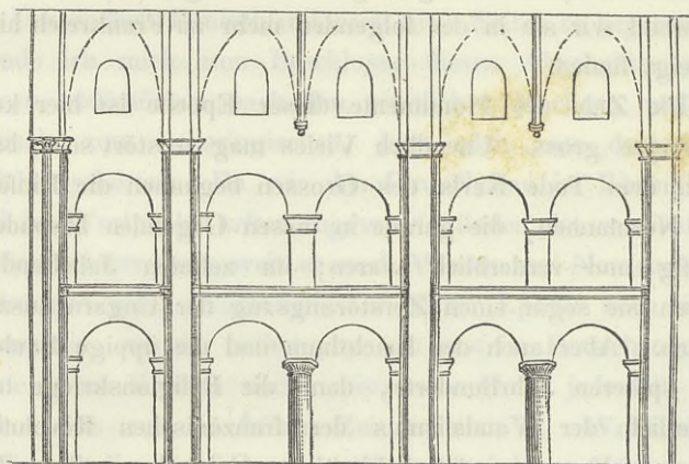
St. Vincent, Soignies.
