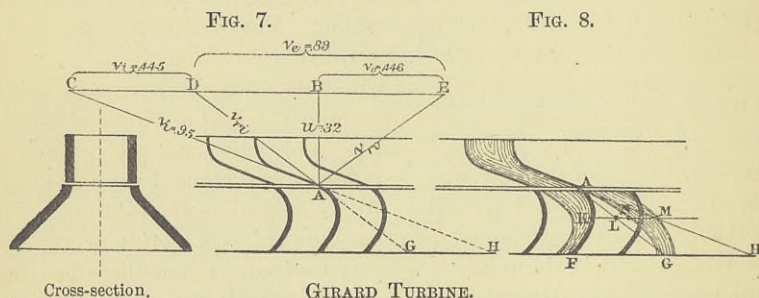
GIRARD TURBINE.
