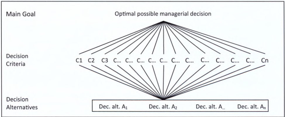
Figure 4.1. Theoretical example of an AHP hierarchical decision-making model Source: Compiled on the basis of Saaty, 1996, pp. 5-6.
