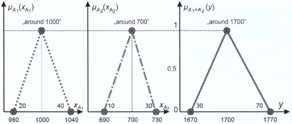
Figure 4.10. Parameters of decision D (Example 4.1), resulting from a sum of two disjoint fuzzy sets – decision alternatives A_1 and A_2 Source: Compiled on the basis of Grzesik (2016, p. 25).
