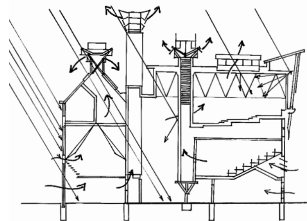
▲ Schemat wentylacji w Queens Building, De Montfort University, Leicester. [1] Scheme of ventilation in the Queens Building, De Montfort University, Leicester.[1]
