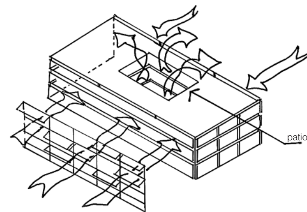
▲ Schemat naturalnej wentylacji w budynku IGuzzini Illuminazione Headquarters, Recanati, Italy.[1] Scheme of natural ventilation in the building of the IGuzzini Illuminazione Headquarters, Recanati, Italy.[1]
